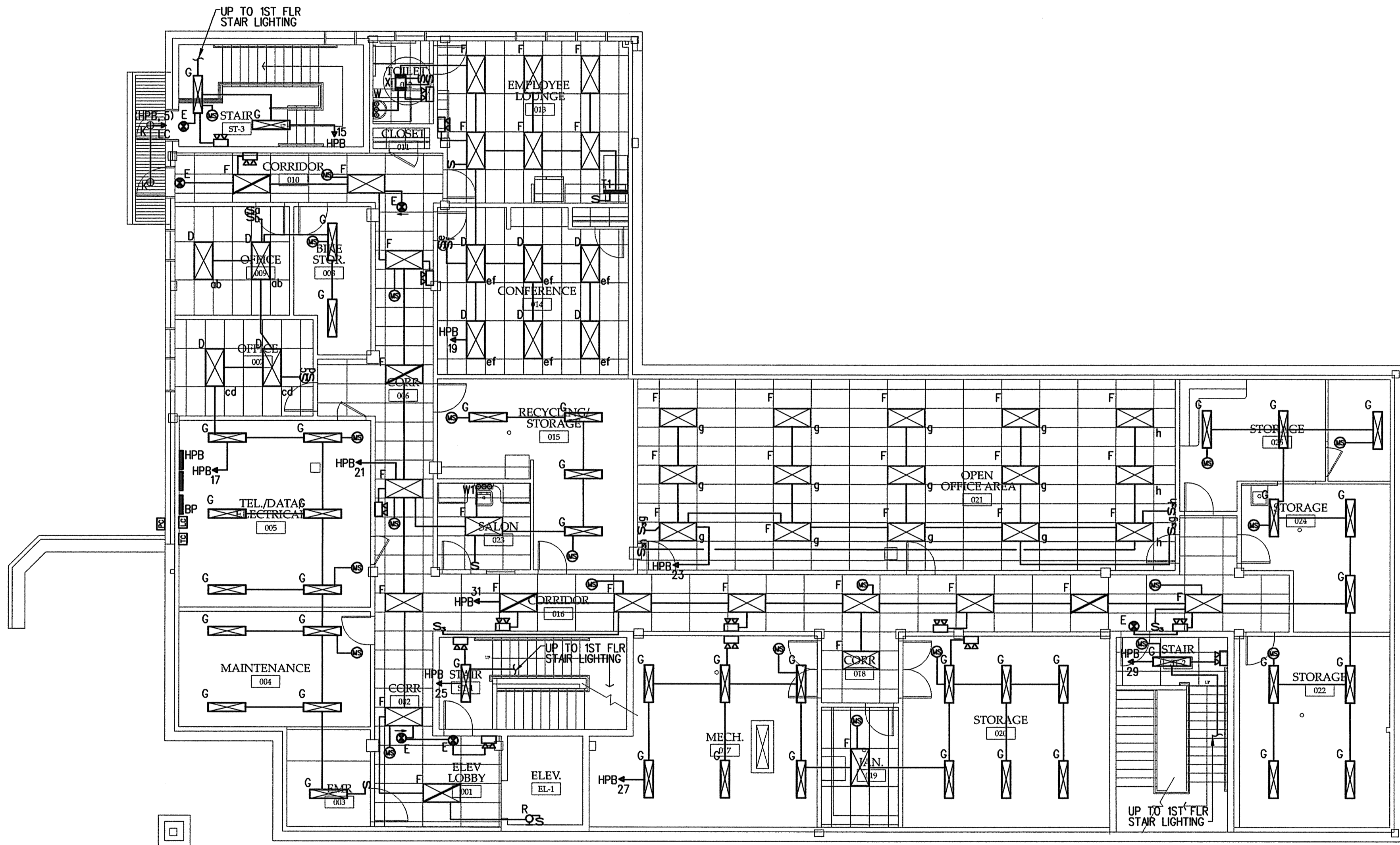
BASEMENT LIGHTING PLAN SCALE: 1/8"=1'-0"
