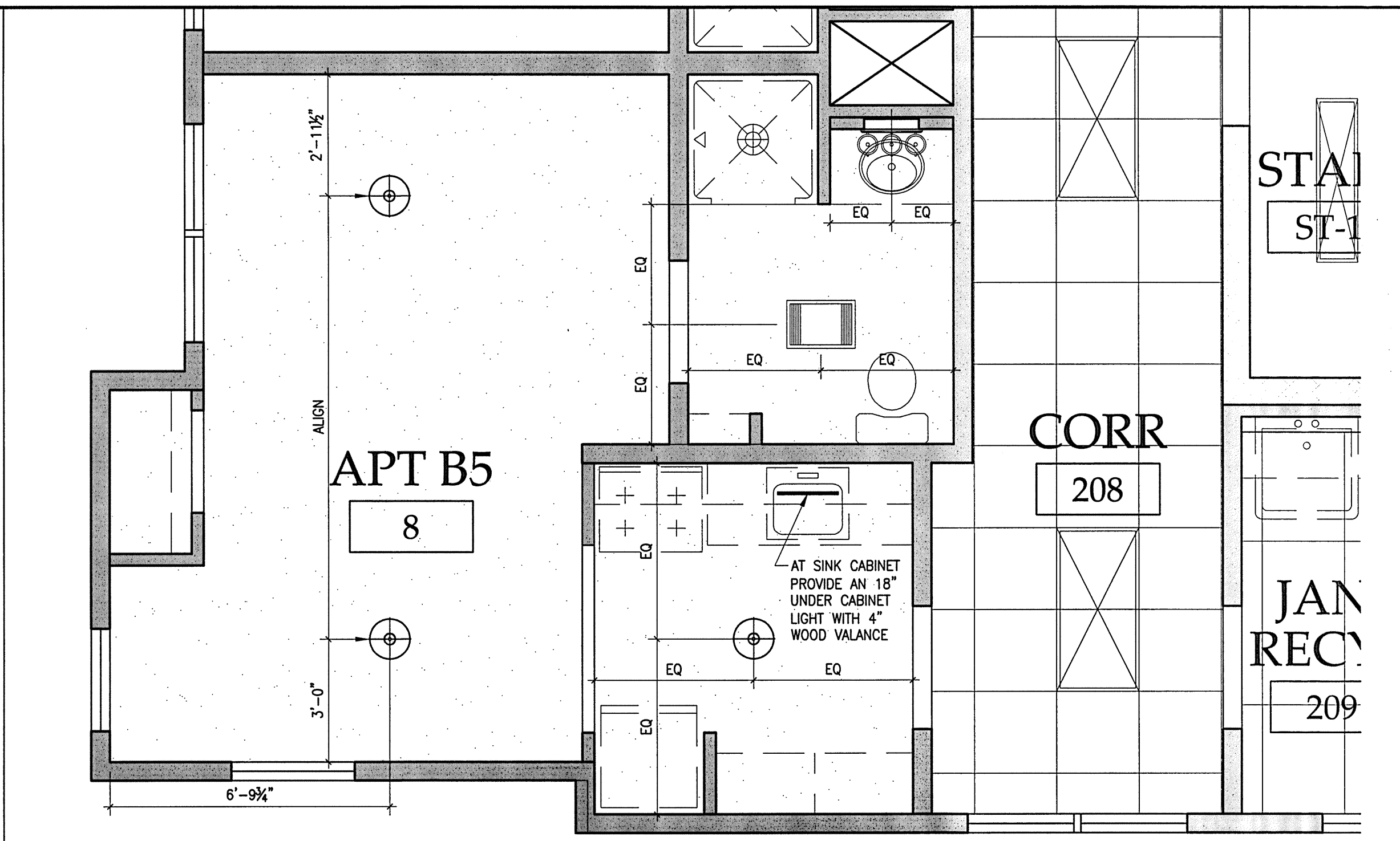
L13 APARTMENT, TYPICAL REFLECTED CEILING PLAN
