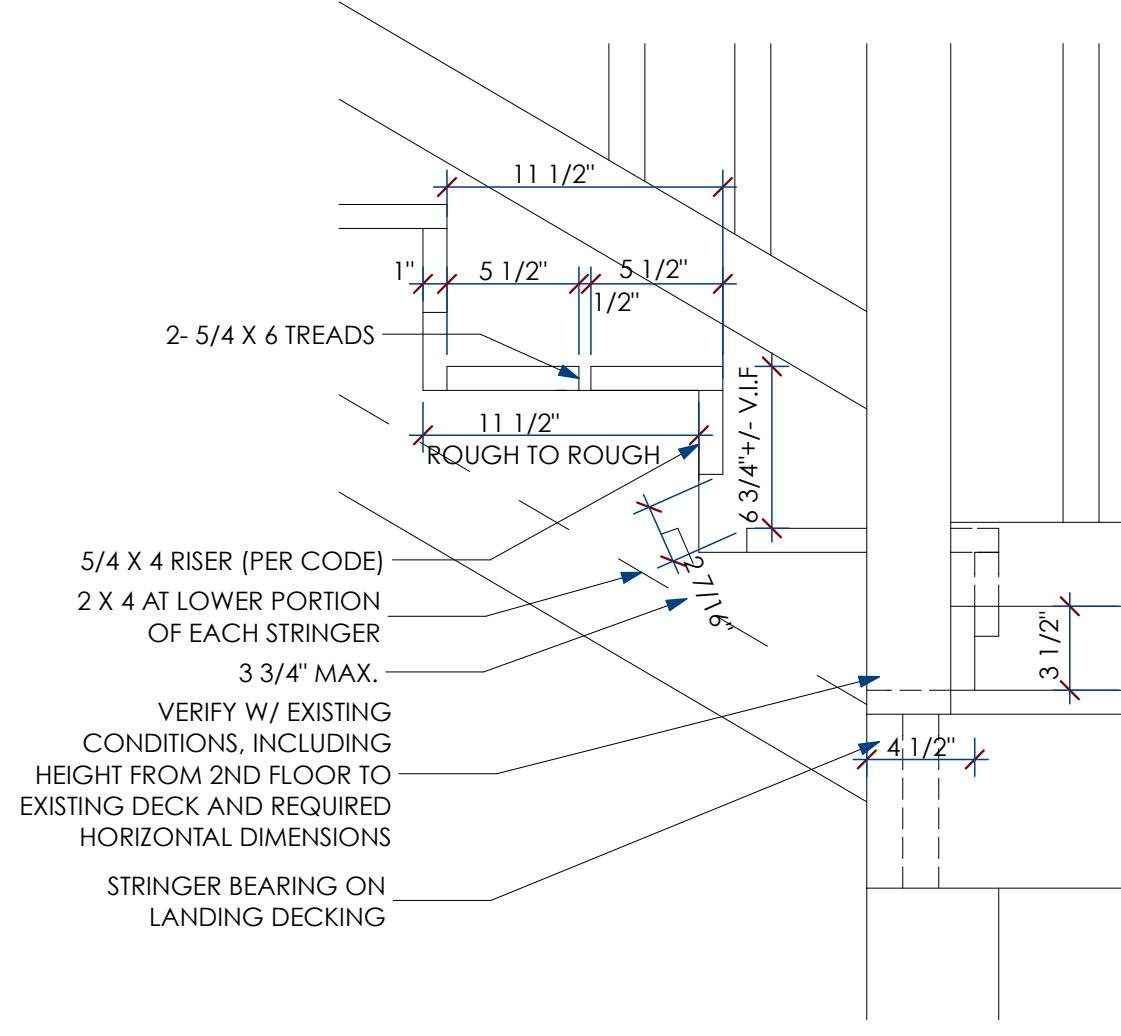
2 STAIR DETAIL- LOWER STAIR RUN SCALE: 1 1/2"= 1'-0"
