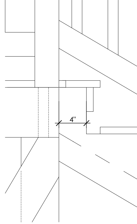
1 STAIR DETAIL- UPPER STAIR RUN SCALE: 1 1/2"= 1'-0"
