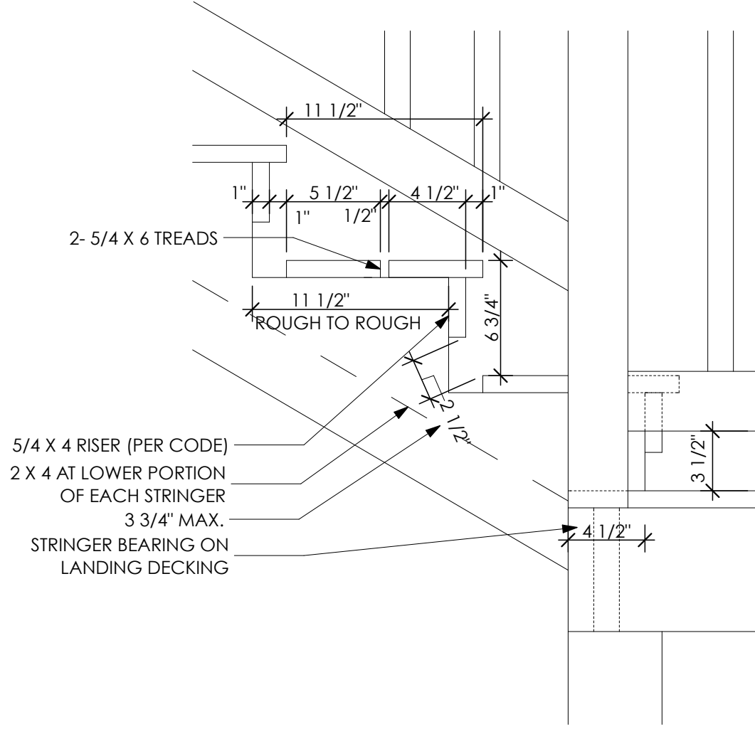
2 STAIR DETAIL- LOWER STAIR RUN SCALE: 1 1/2"= 1'-0"
