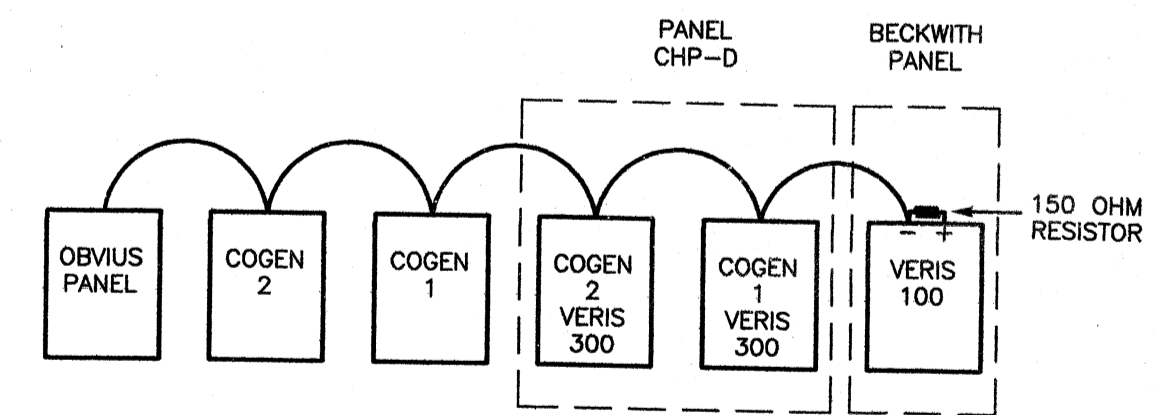
DATA LOOP DETAIL RS 485 ORDER SCALE: NONE
