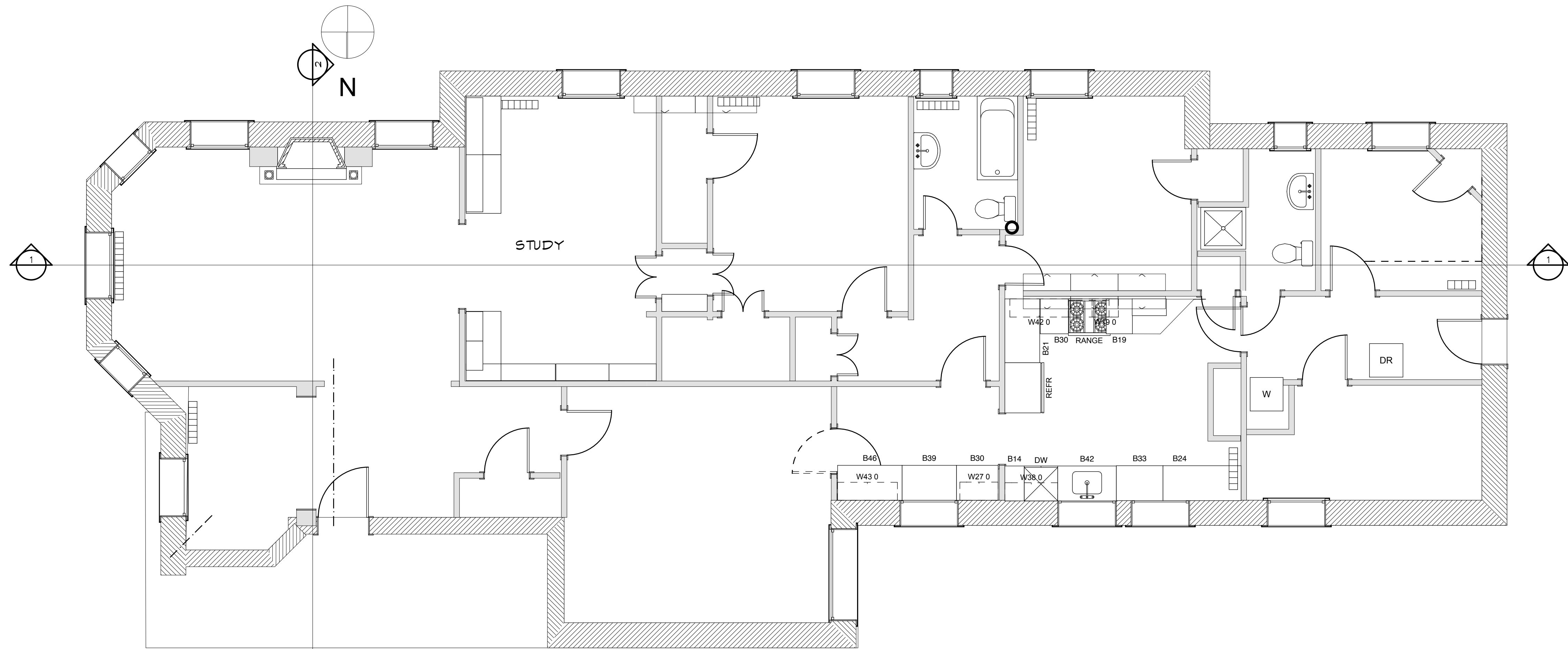
EXISTING PLAN
