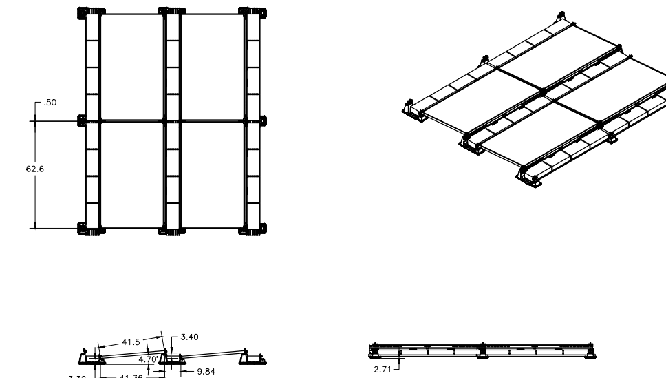
PANASONIC 330W ECOFOOT5D LANDSCAPE ELEVATION/ISO VIEWS SCALE: NTS UNITS: INCHES
