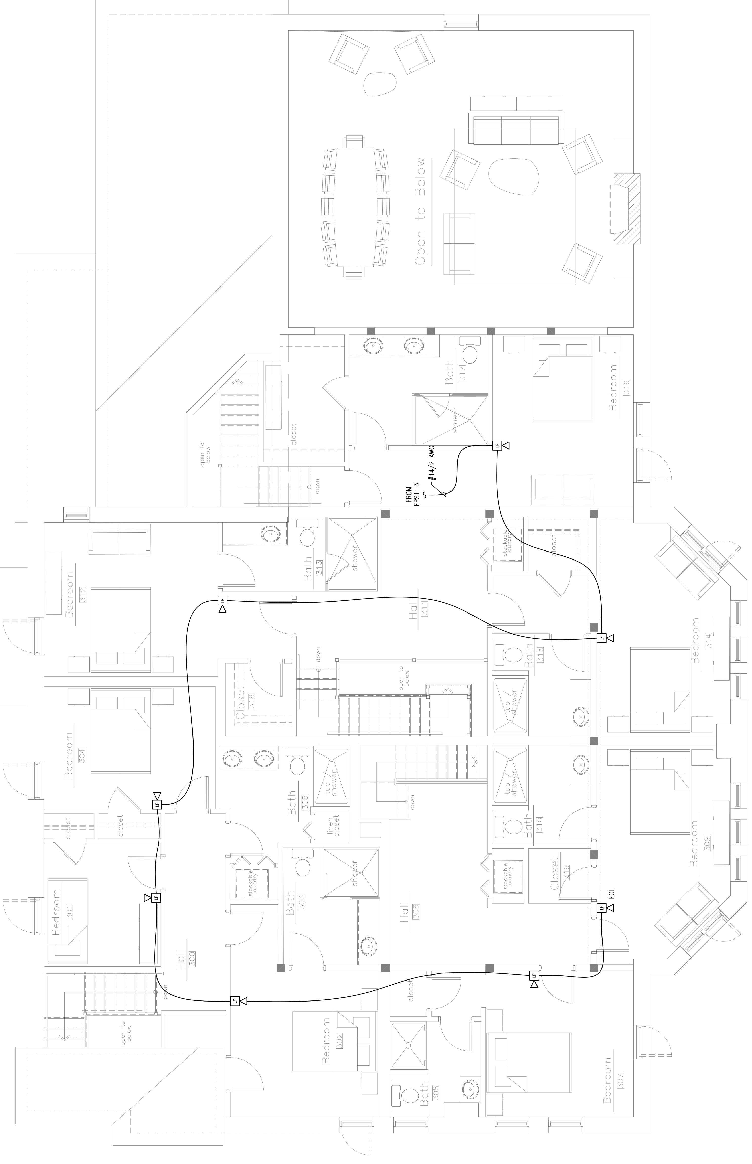
THIRD FLOOR FIRE ALARM PLAN SCALE: 1/4"=1'-0"
