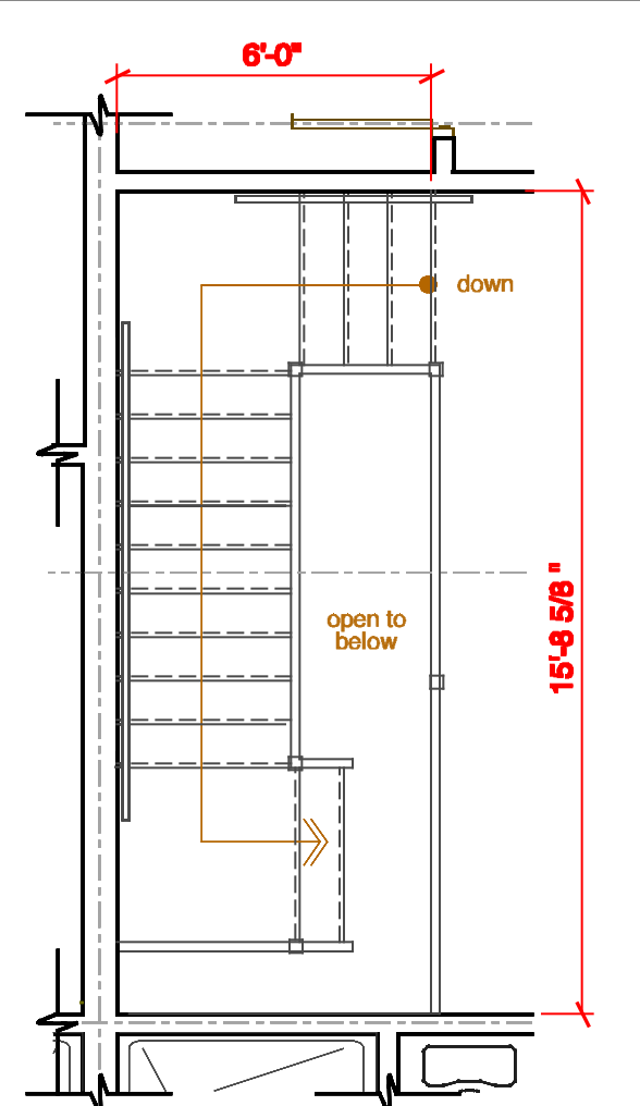
32 3rd Floor Plan Scale: 1/4" = 1'-0"
