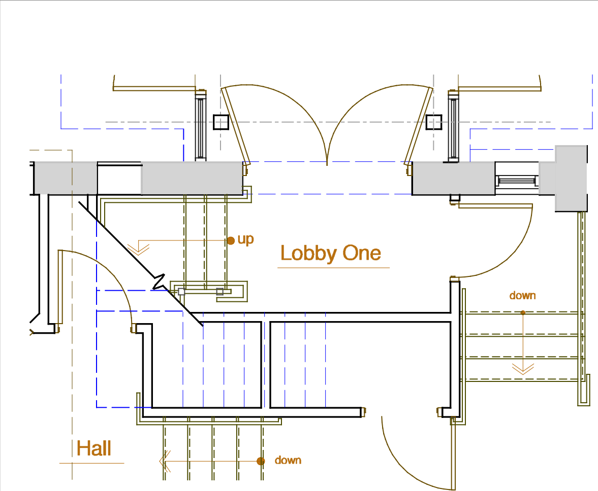
12 1st Floor Plan Scale: 1/4" = 1'-0"
