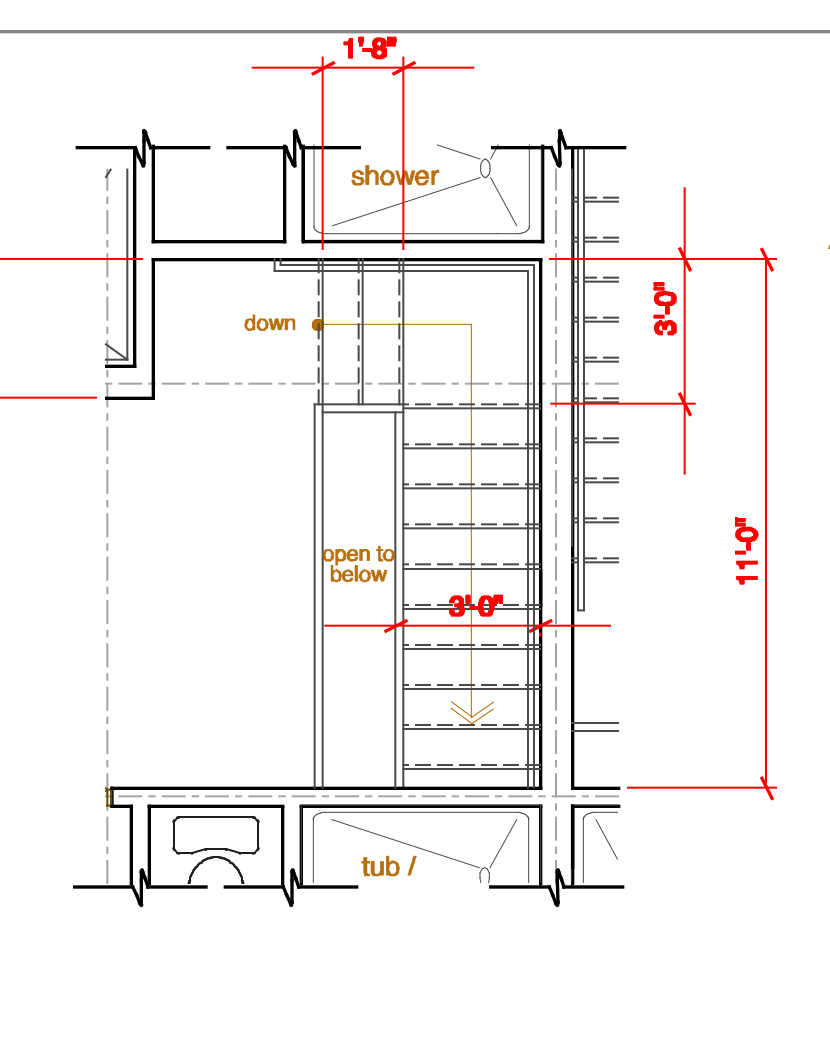
42 3rd Floor Plan Scale: 1/4" = 1'-0"
