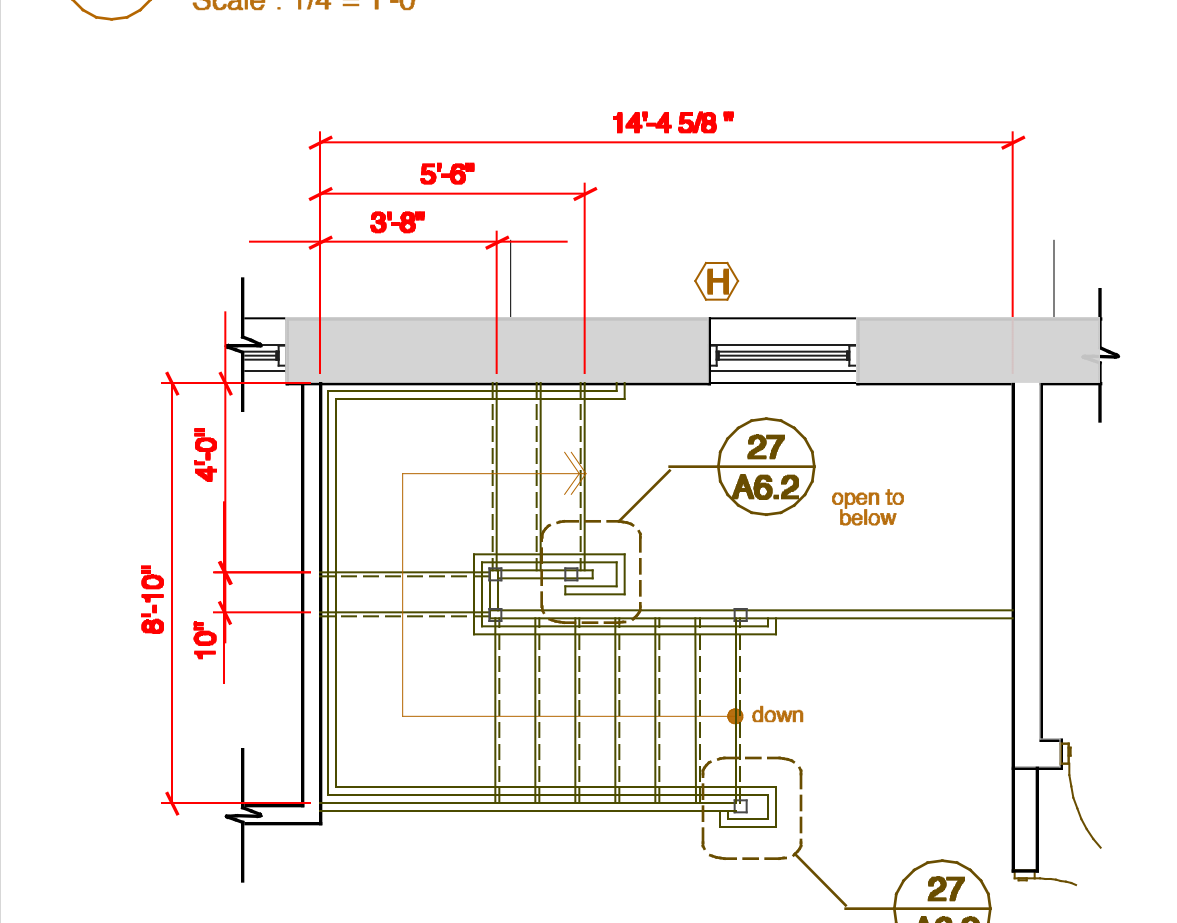
11 2nd Floor Plan Scale: 1/4" = 1'-0"
