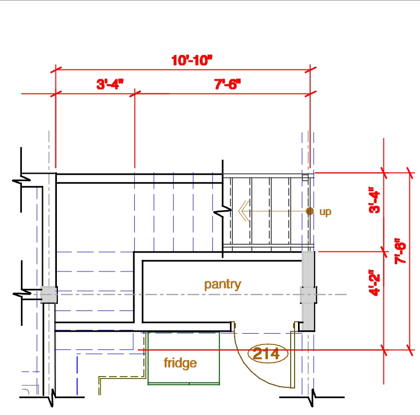
23 2nd Floor Plan Scale: 1/4" = 1'-0"
