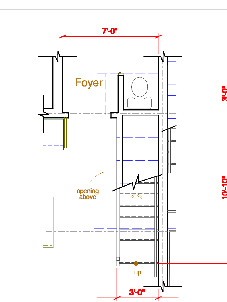
43 2nd Floor Plan Scale: 1/4" = 1'-0"
