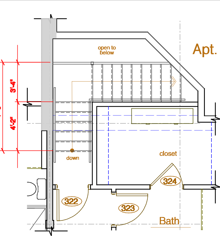
22 3rd Floor Plan Scale: 1/4" = 1'-0"
