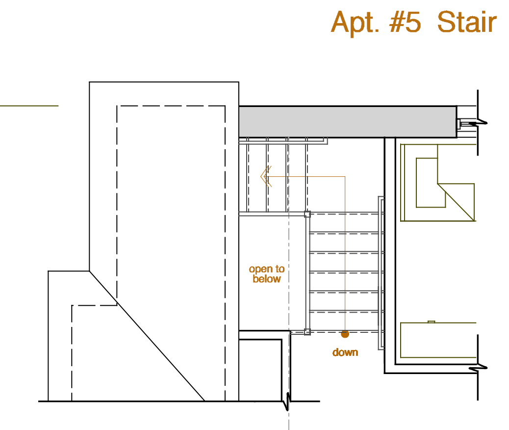
52 3rd Floor Plan Scale: 1/4" = 1'-0"
