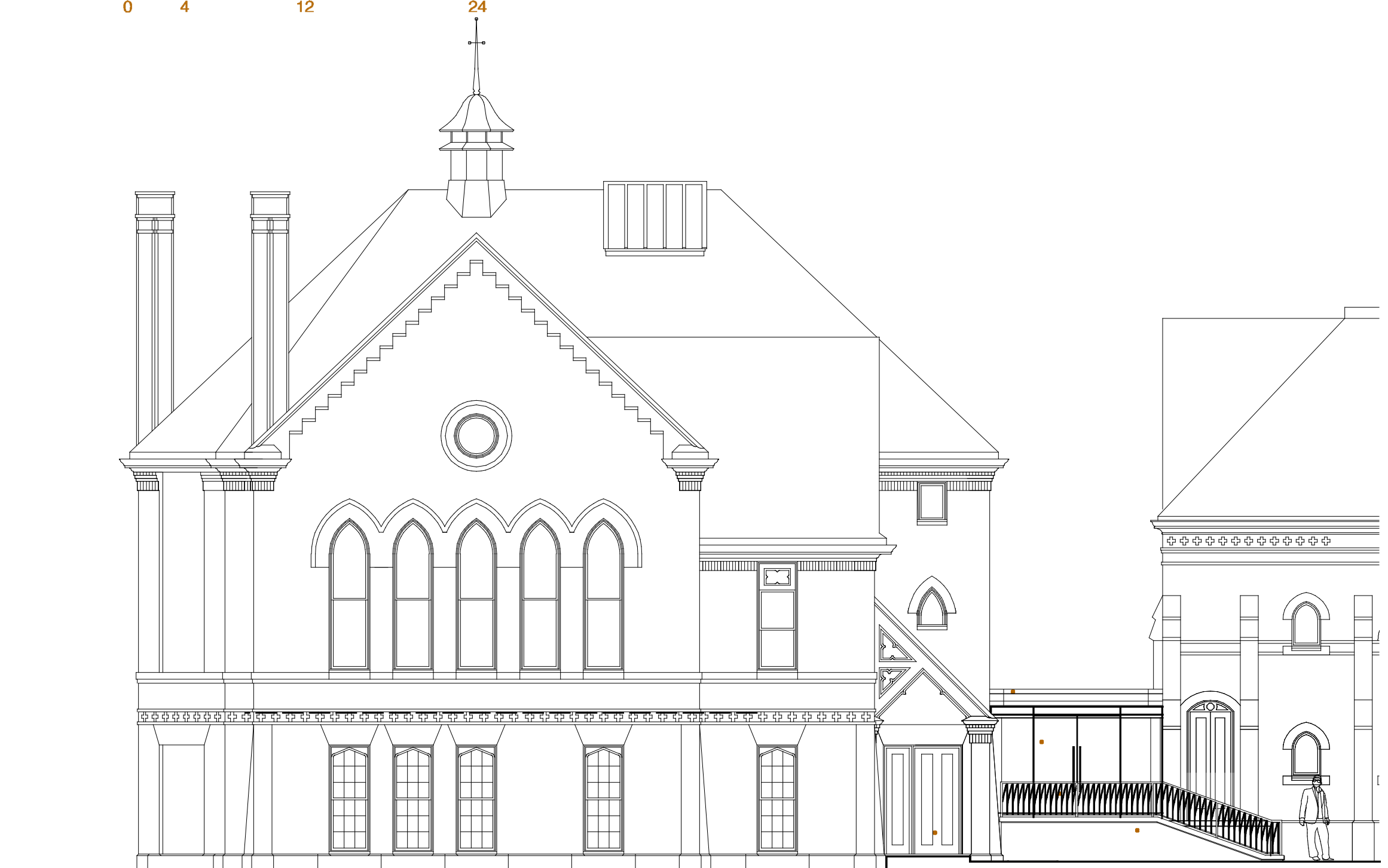
11 South Elevation
