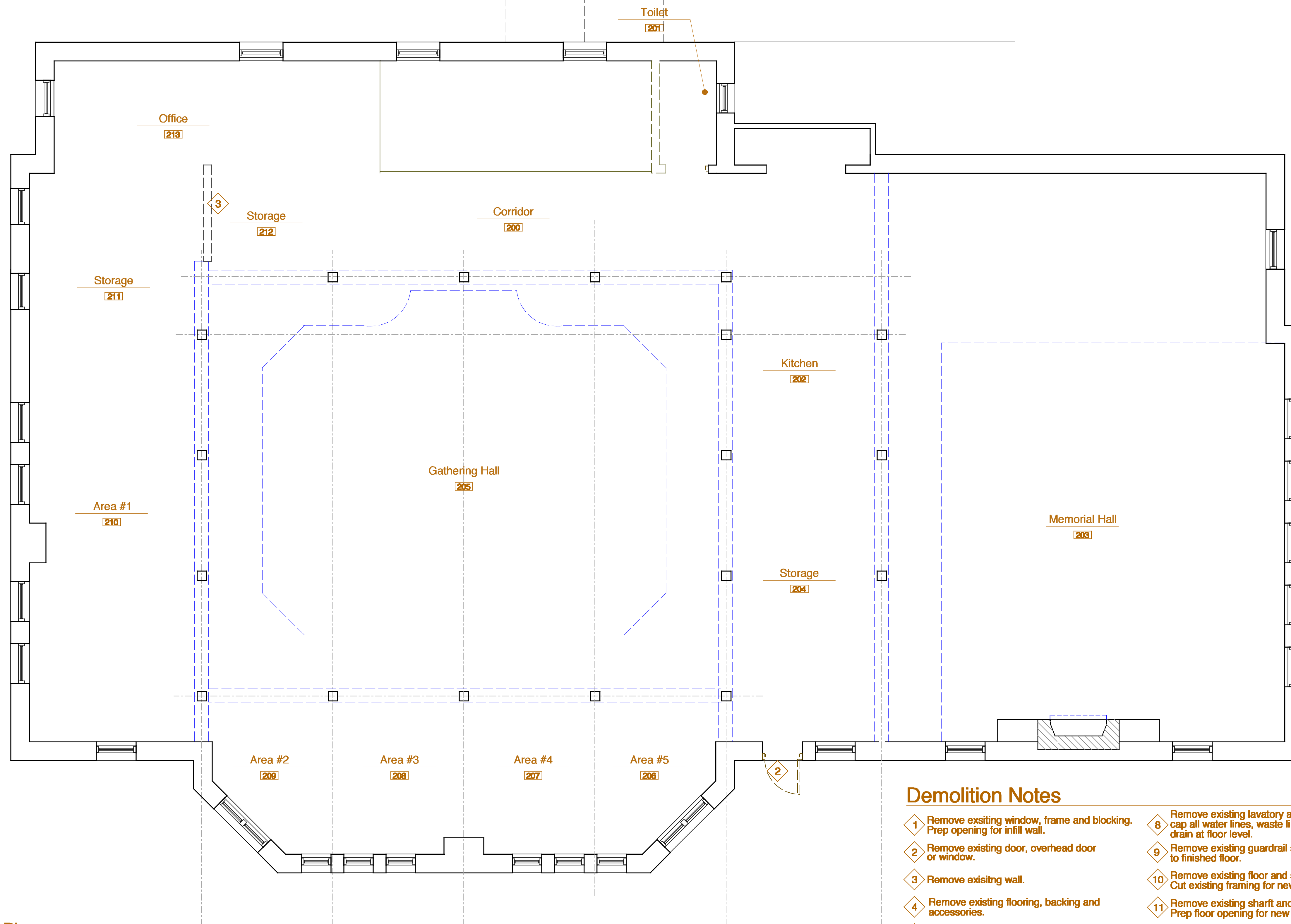
10 Second Floor Demolition Plan 0 4 12 24
