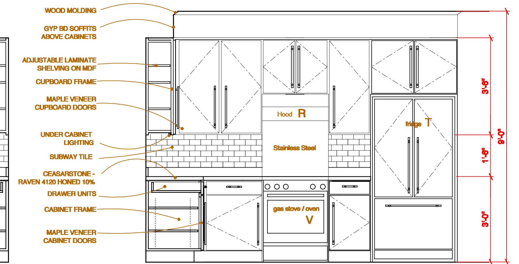
42 Unit #4 Kitchen Elevation Scale: 1/2"=1'-0"
