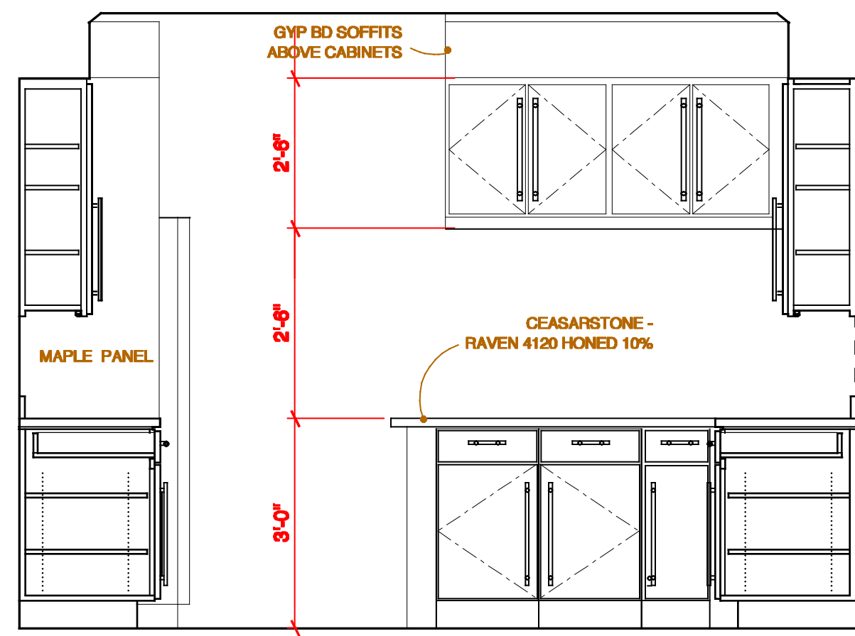
50 Unit #5 Kitchen Elevation Scale: 1/2"=1'-0"
