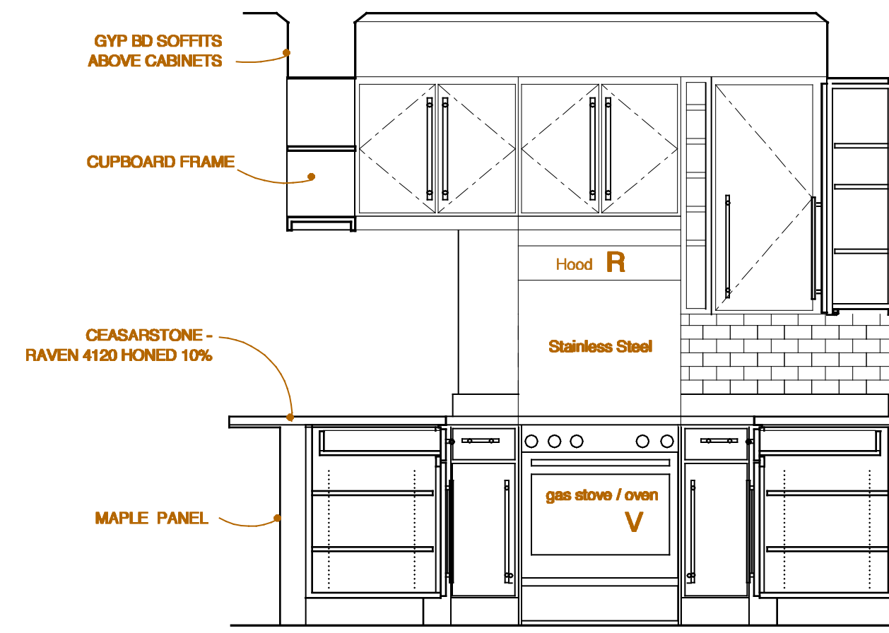
51 Unit #5 Kitchen Elevation Scale: 1/2"=1'-0"
