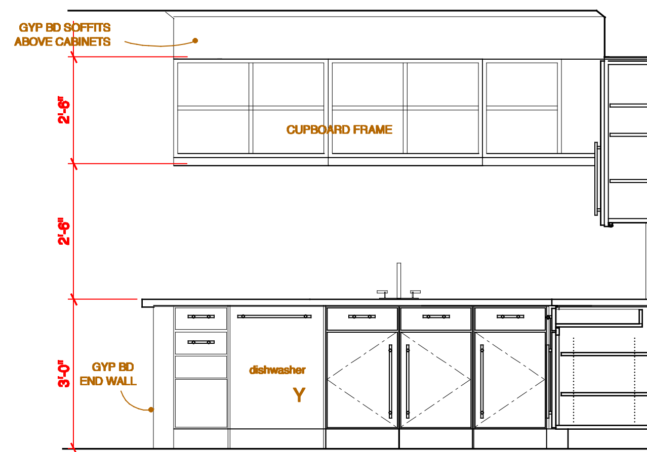
40 Unit #4 Kitchen Elevation Scale: 1/2"=1'-0"
