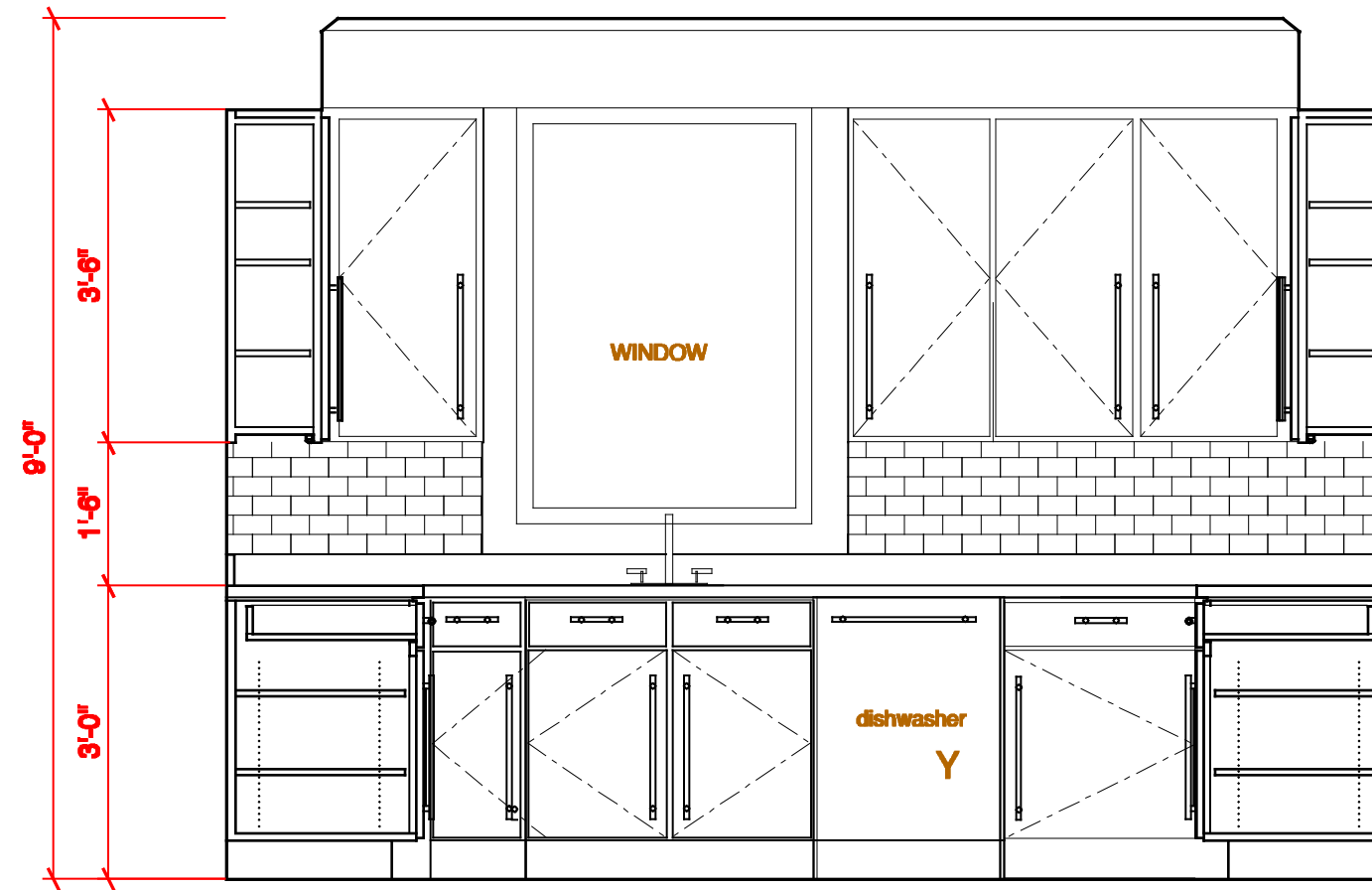
52 Unit #5 Kitchen Elevation Scale: 1/2"=1'-0"
