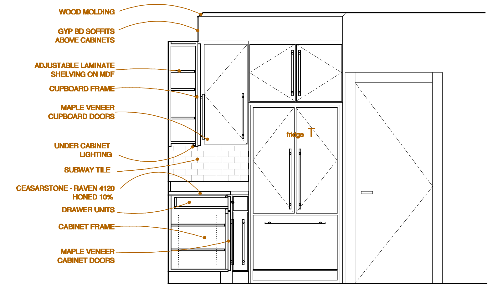
53 Unit #5 Kitchen Elevation Scale: 1/2"=1'-0"
