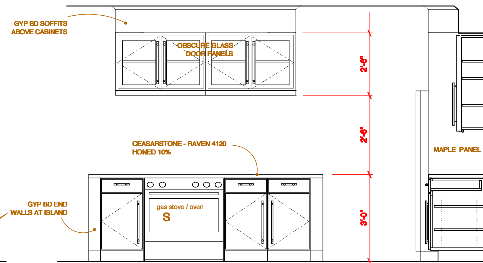
31 Unit #3 Kitchen Elevation Scale: 1/2"=1'-0"
