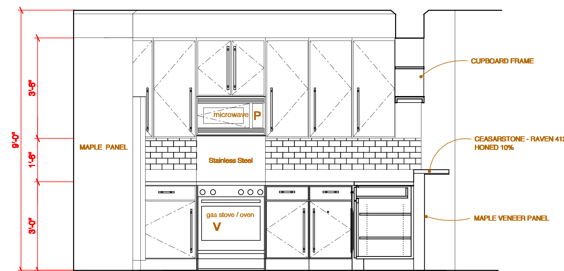
10 Unit #1 Kitchen Elevation Scale: 1/2"=1'-0"
