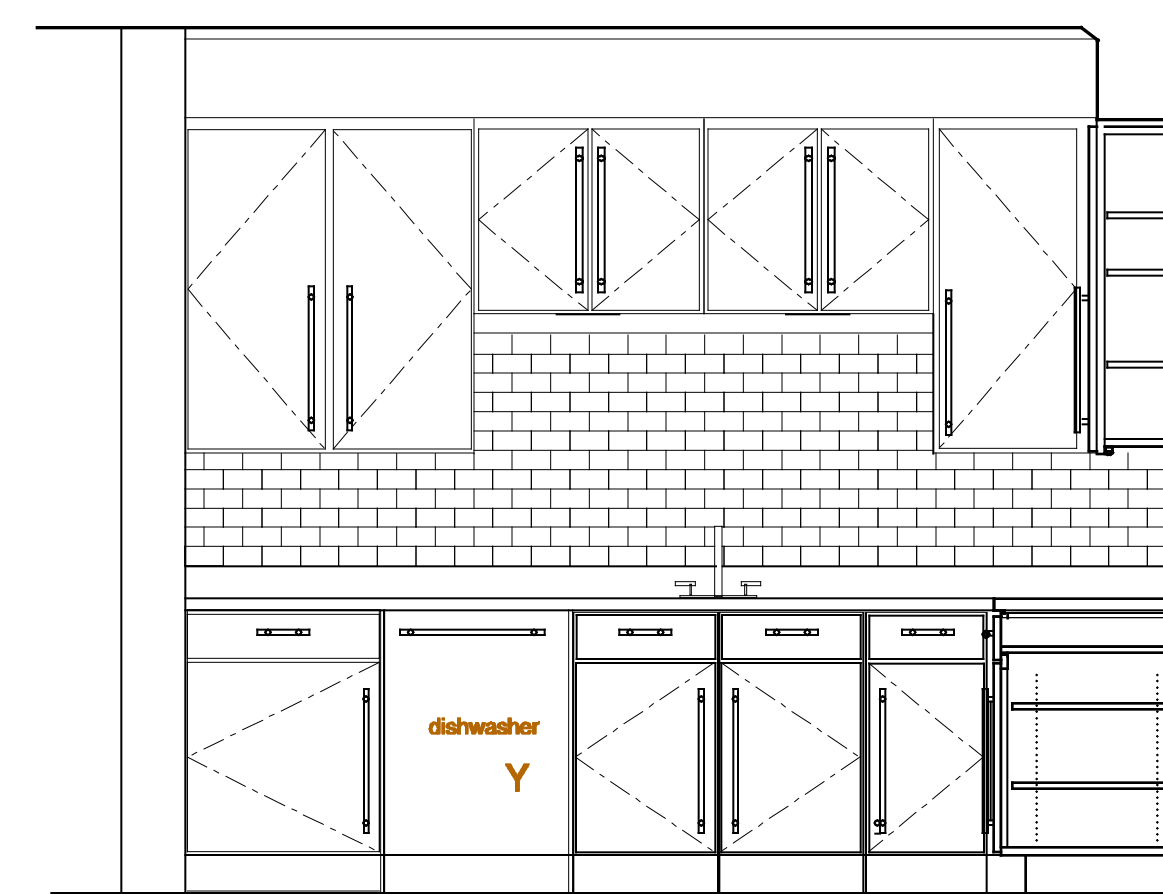
20 Unit #2 Kitchen Elevation Scale: 1/2"=1'-0"
