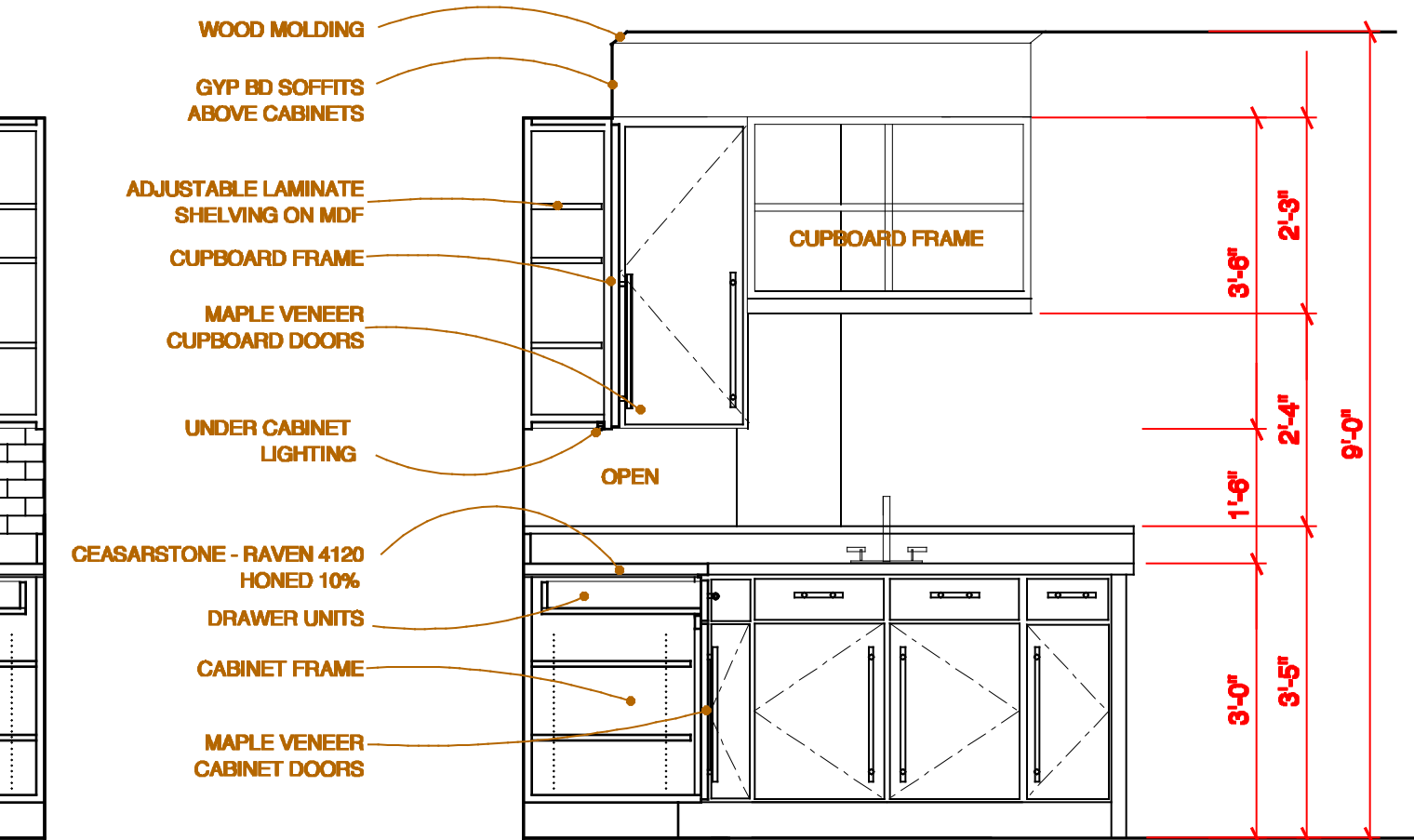
12 Unit #1 Kitchen Elevation Scale: 1/2"=1'-0"
