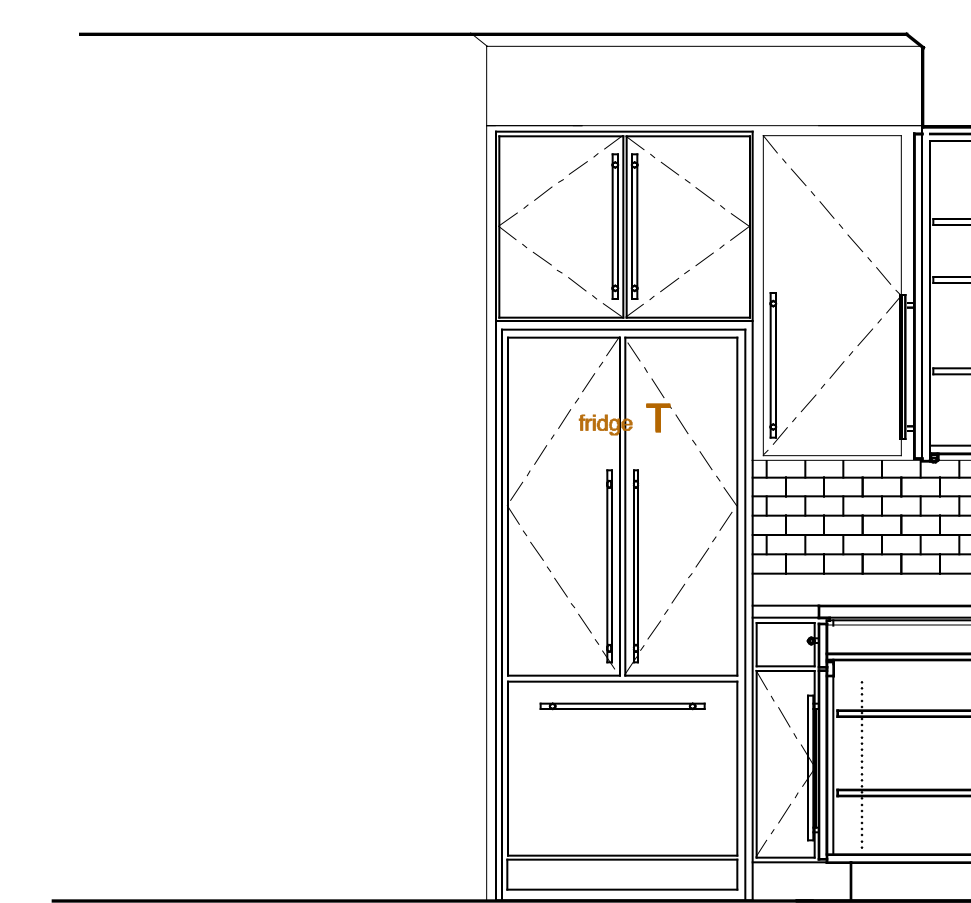
11 Unit #1 Kitchen Elevation Scale: 1/2"=1'-0"
