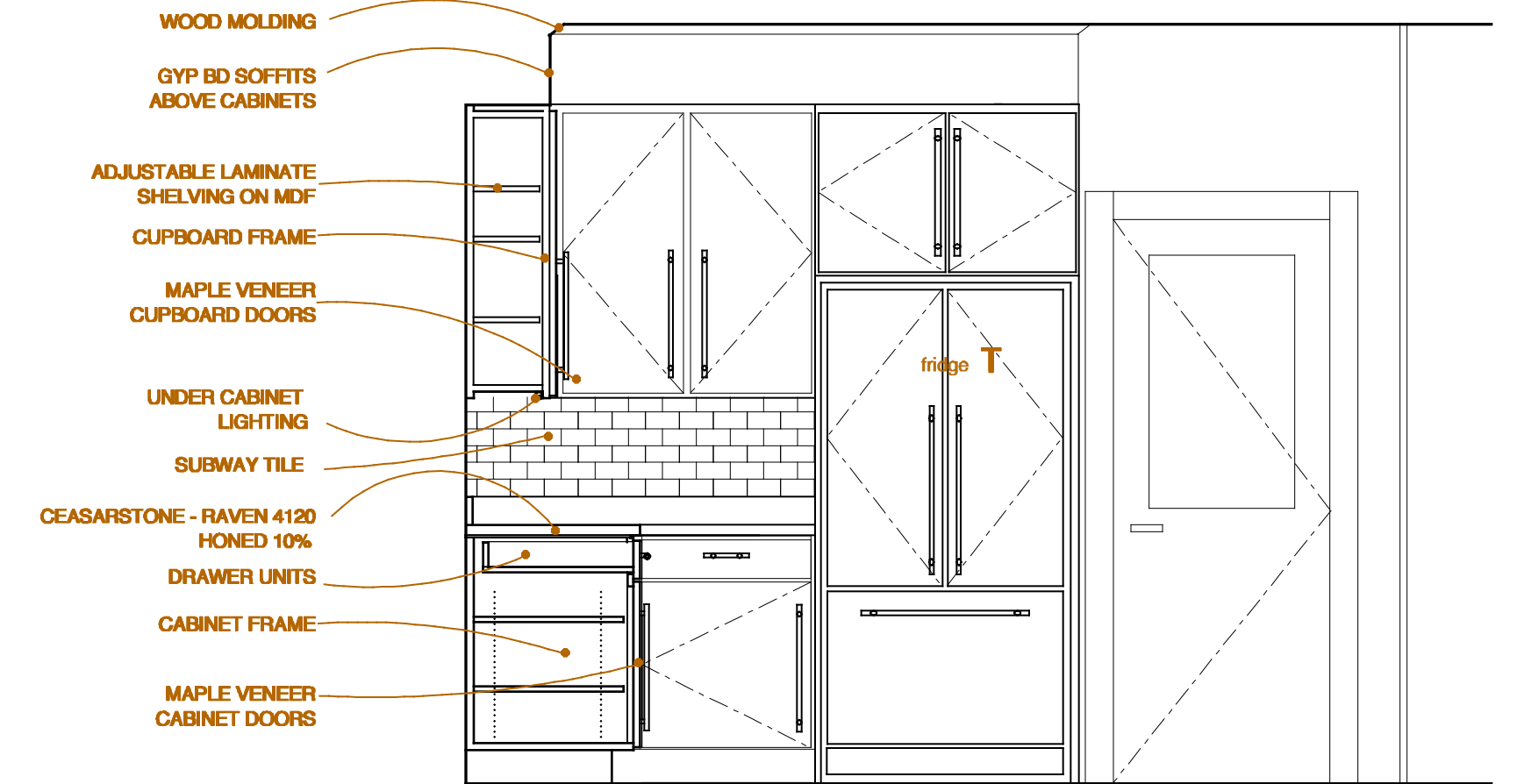
22 Unit #2 Kitchen Elevation Scale: 1/2"=1'-0"
