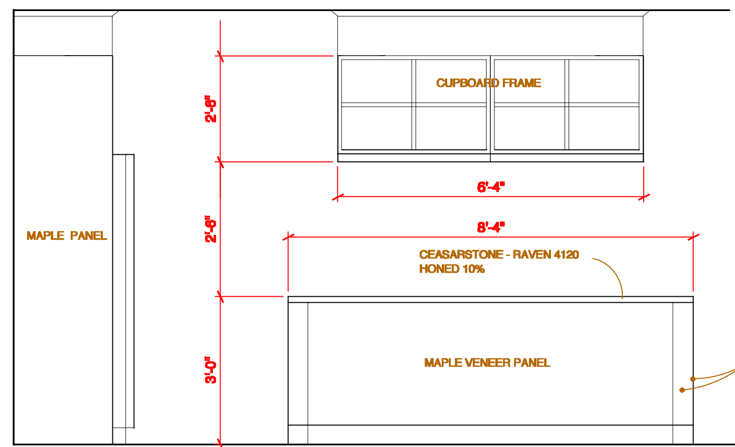
30 Unit #3 Kitchen Elevation Scale: 1/2"=1'-0"
