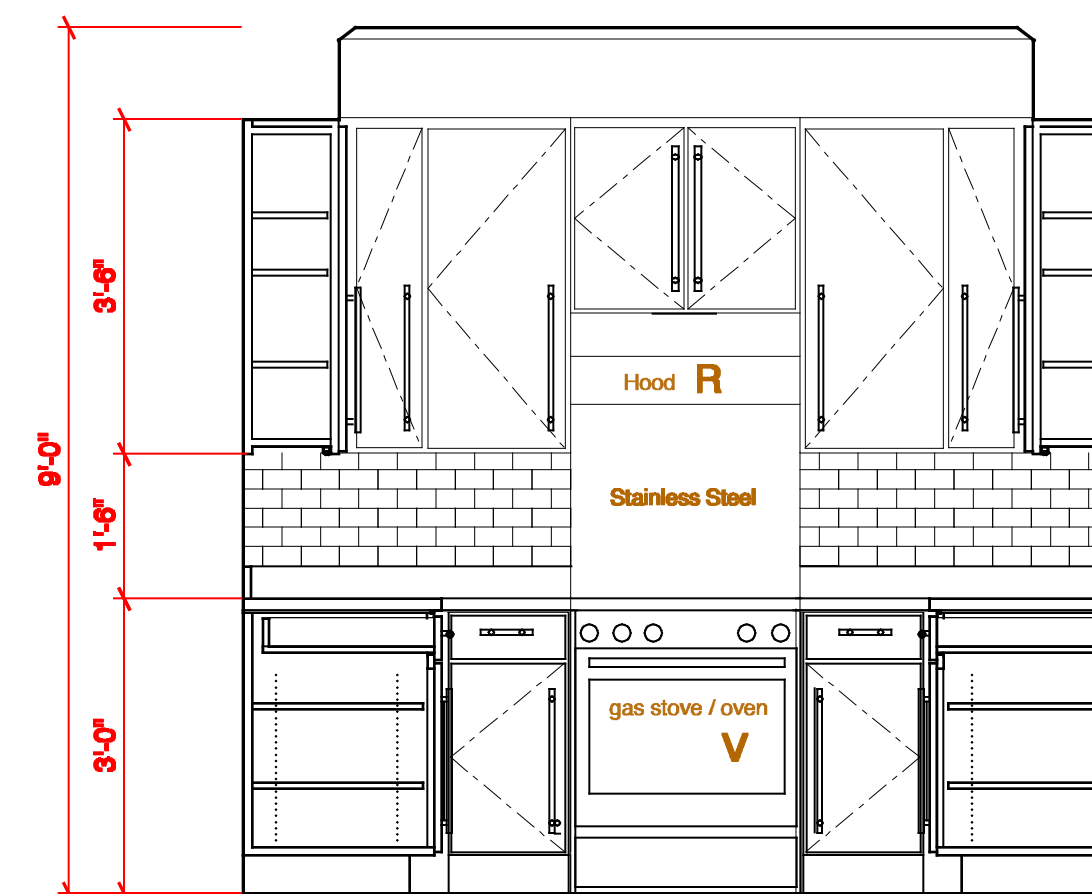
21 Unit #2 Kitchen Elevation Scale: 1/2"=1'-0"
