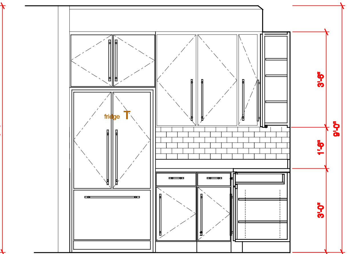
33 Unit #3 Kitchen Elevation Scale: 1/2"=1'-0"
