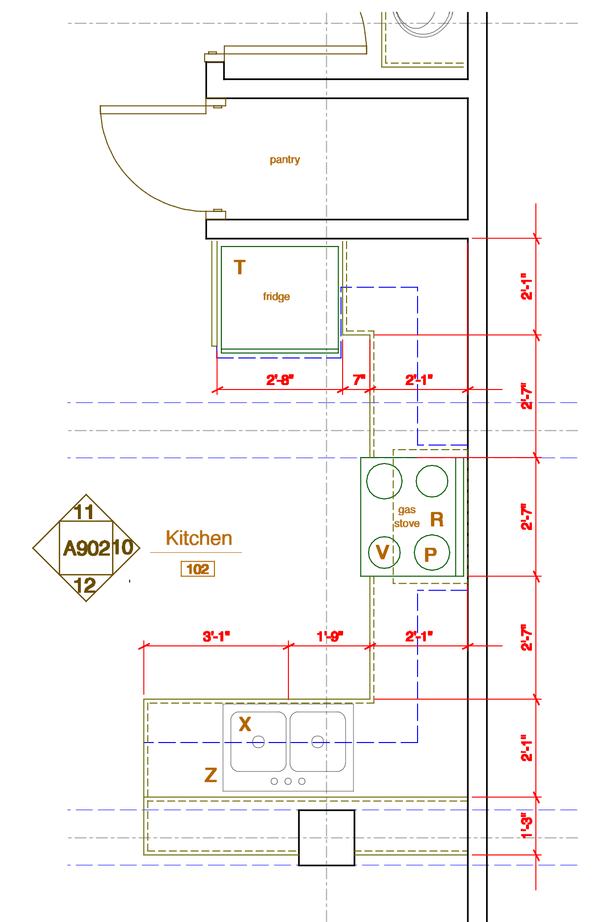
10 Unit #1 (Caretaker) Enlg'd Kitchen Plan
