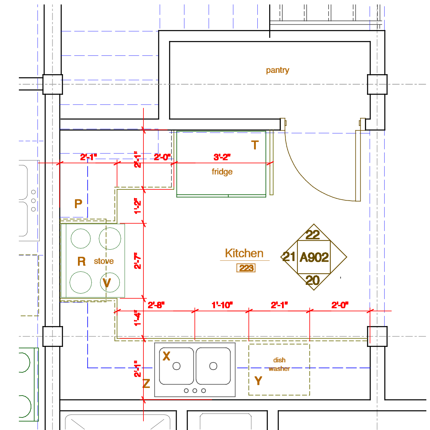
11 Unit #2 Enlarged Kitchen Plan
