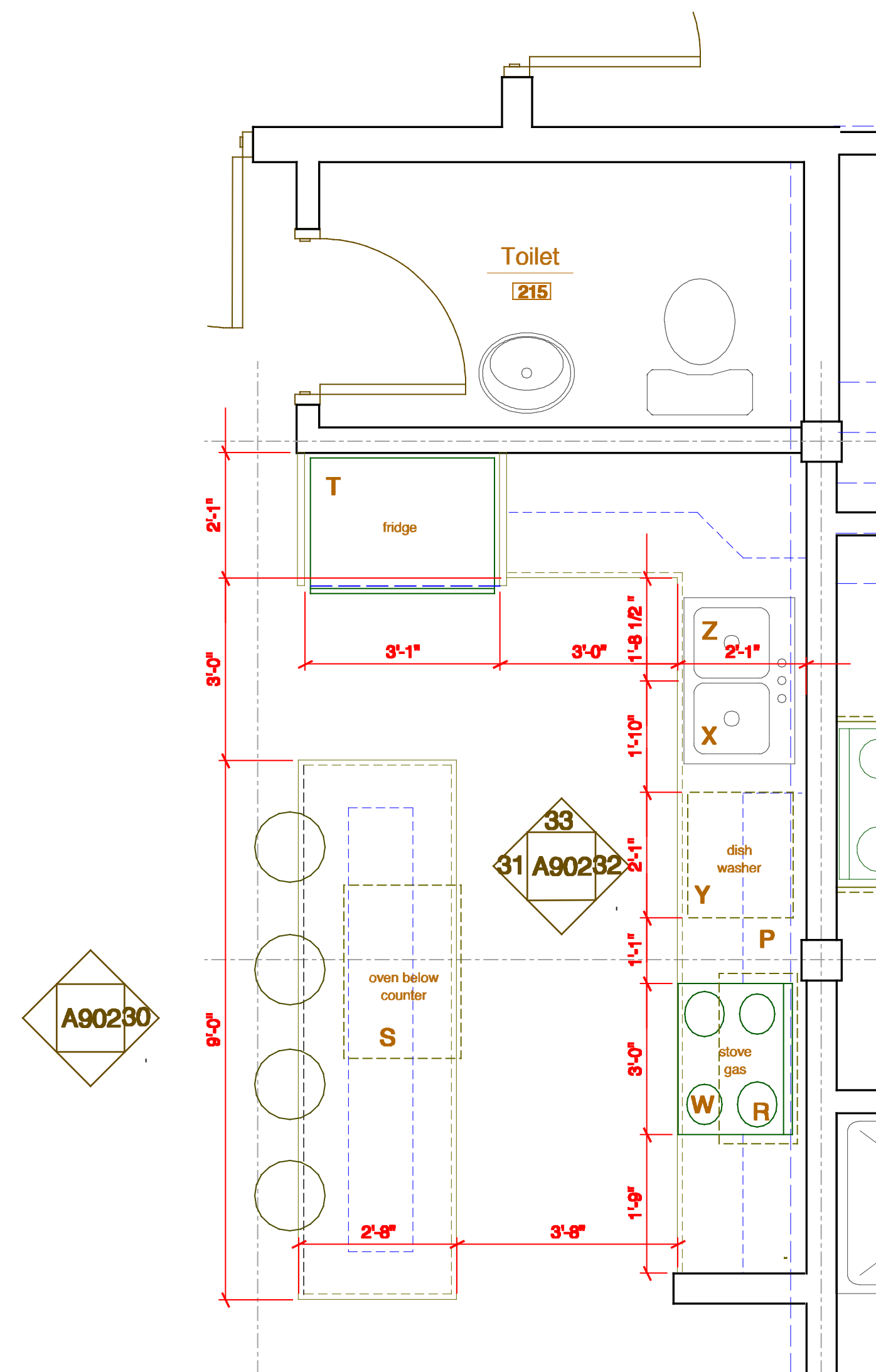
20 Unit #3 Enlarged Kitchen Plan
