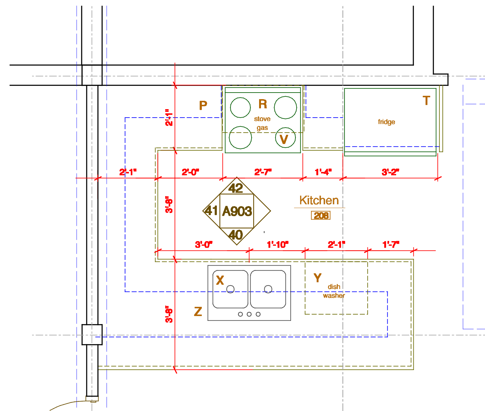
21 Unit #4 Enlarged Kitchen Plan
