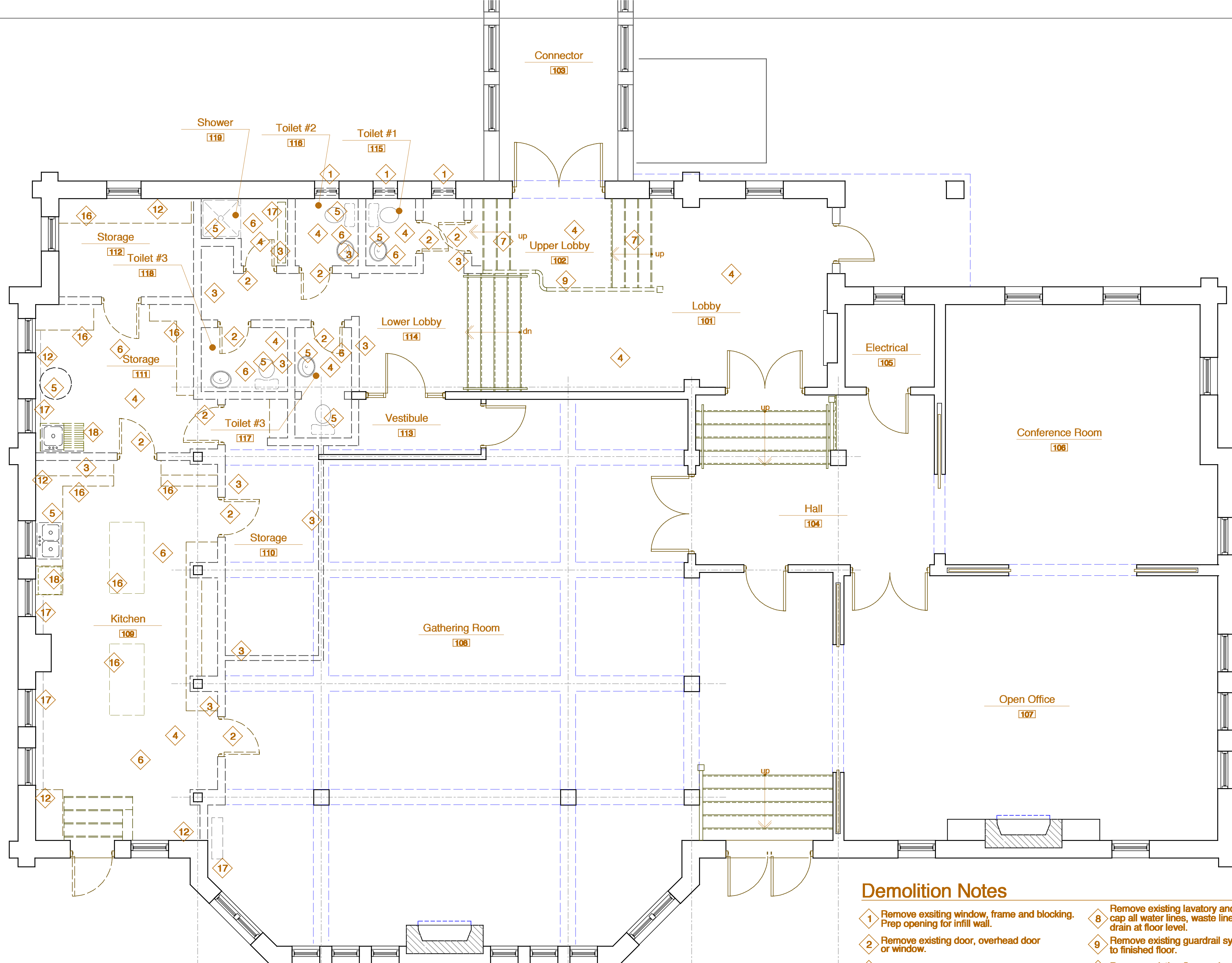
10 First Floor Demolition Plan 0 4 12 24
