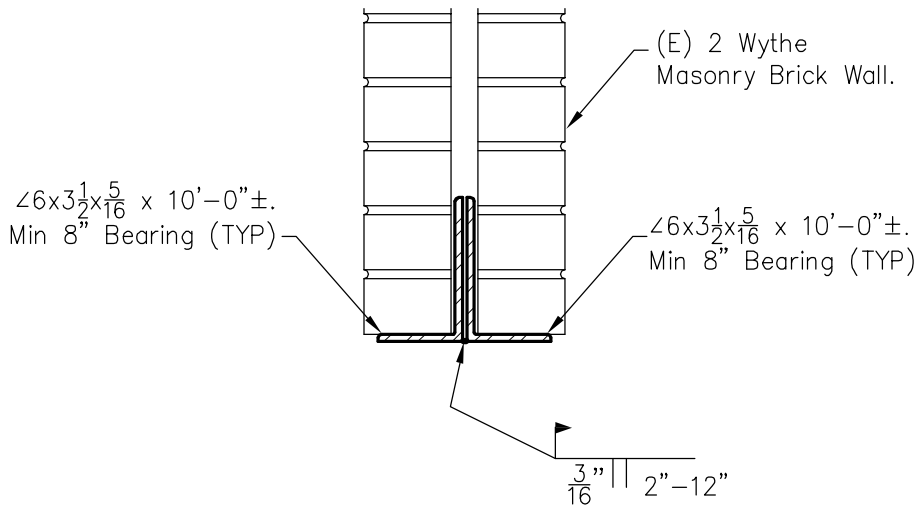
DETAIL BEAM DETAIL
