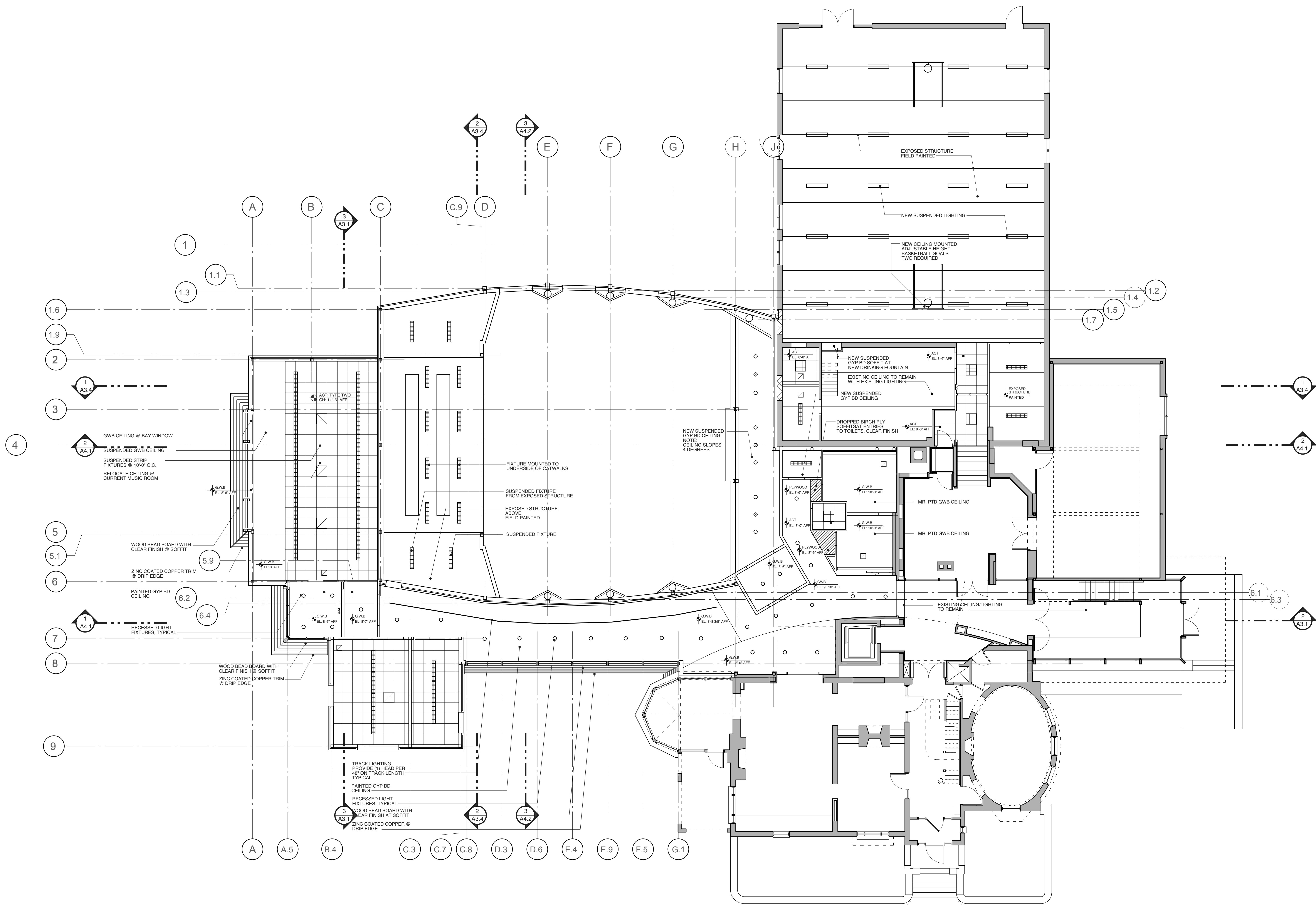
1 FIRST FLOOR REFLECTED CEILING PLAN SCALE: 1/8" = 1'-0"
