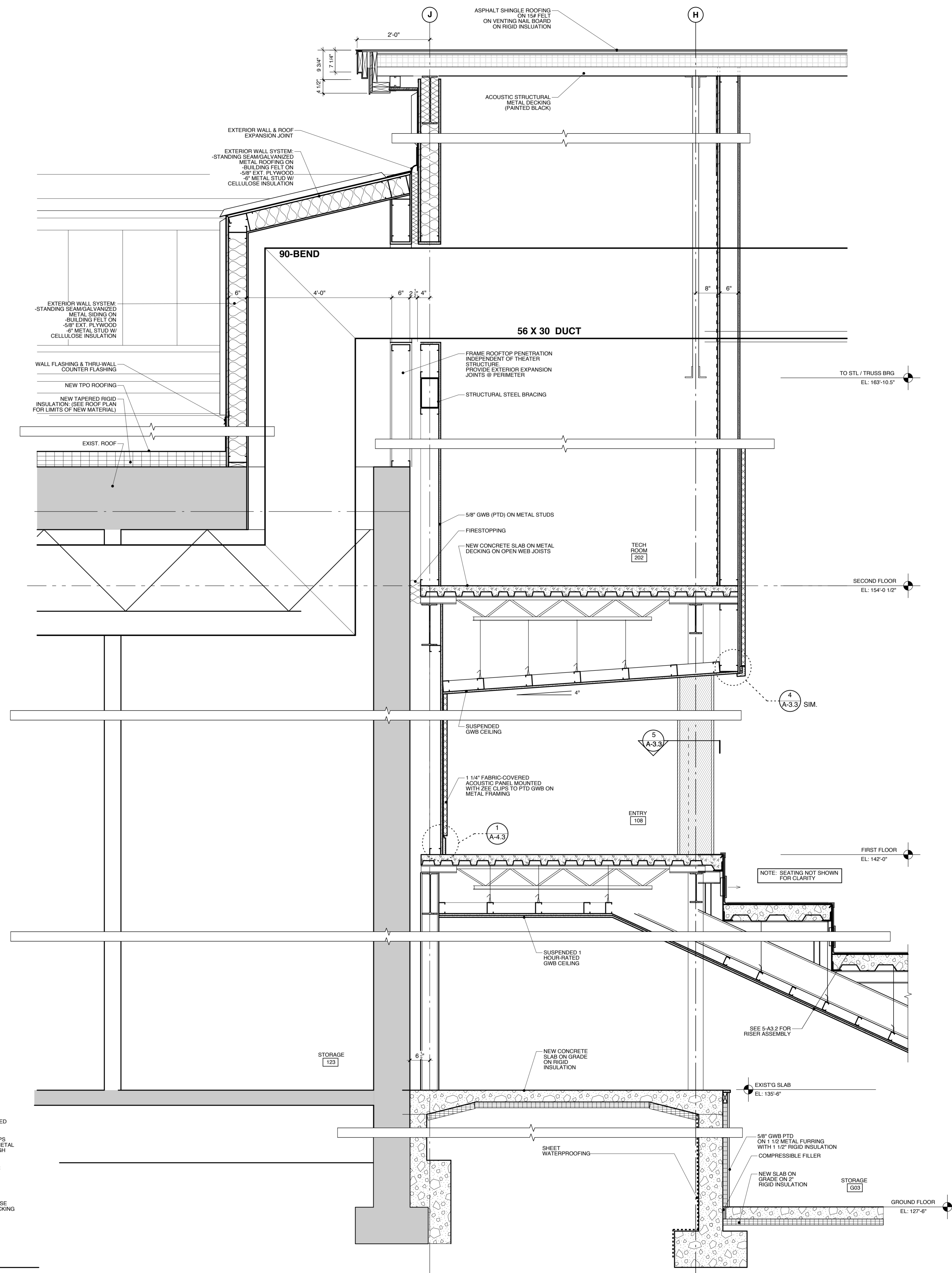
2 WALL SECTION @ JOINT OF OLD / NEW CONSTRUCTION SCALE: 3/4" = 1'-0"
