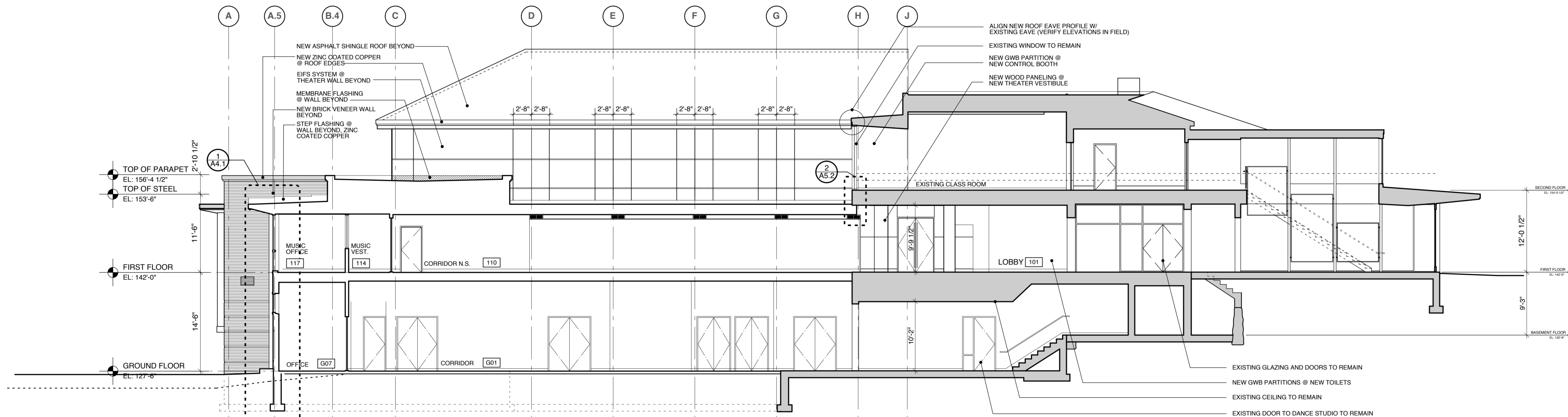
2 BUILDING SECTION SCALE: 1/8" = 1'-0"
