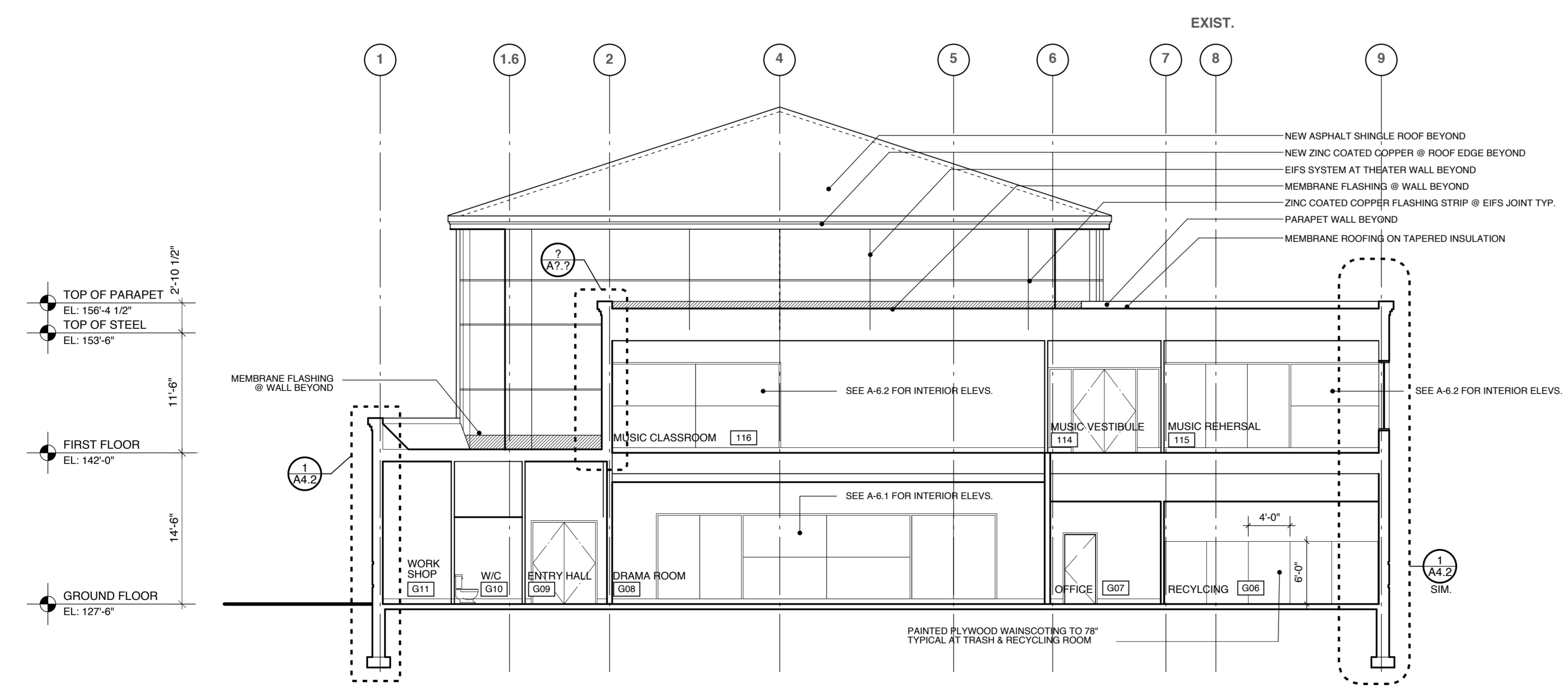
3 BUILDING SECTION SCALE: 1/8" = 1'-0"
