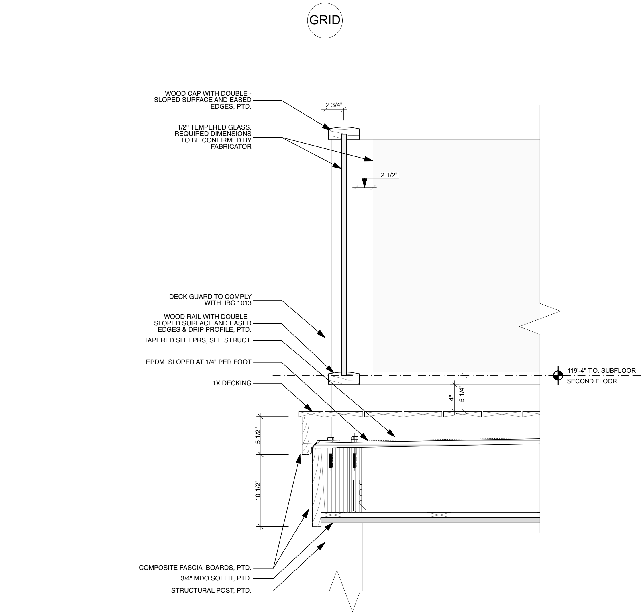
2 EAST DECK-RAIL AND DECK DETAIL SCALE: 1 1/2" = 1'-0"
