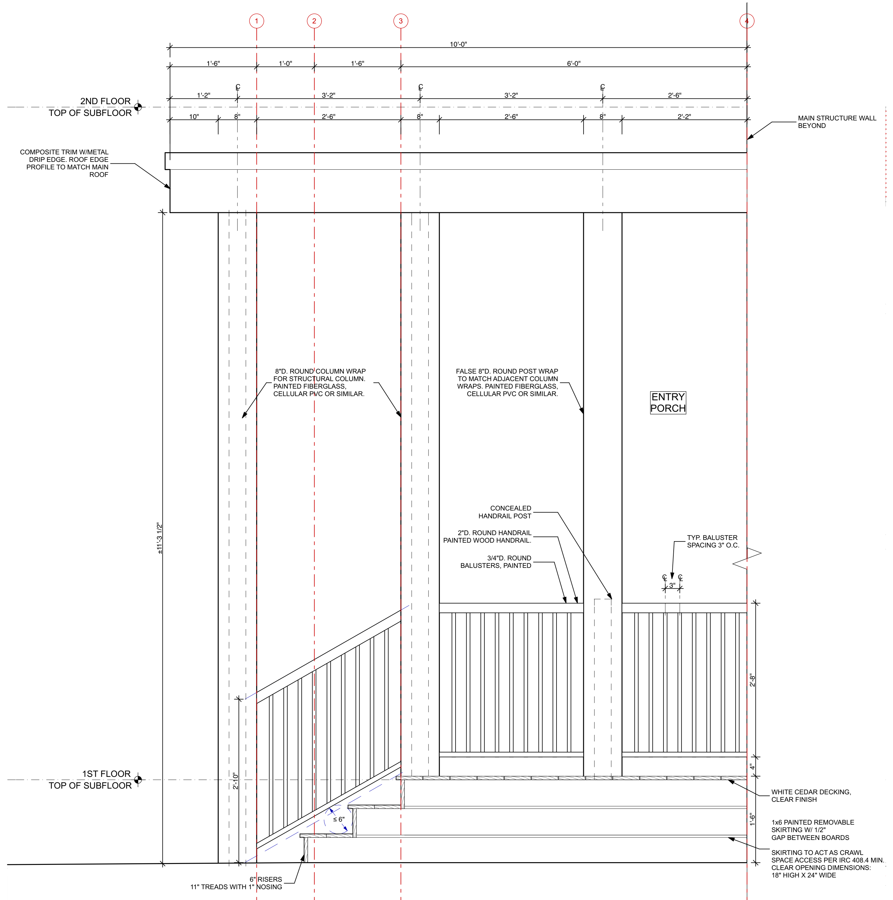
4 ENTRY BALUSTER SECTION SCALE: 1" = 1'-0"
