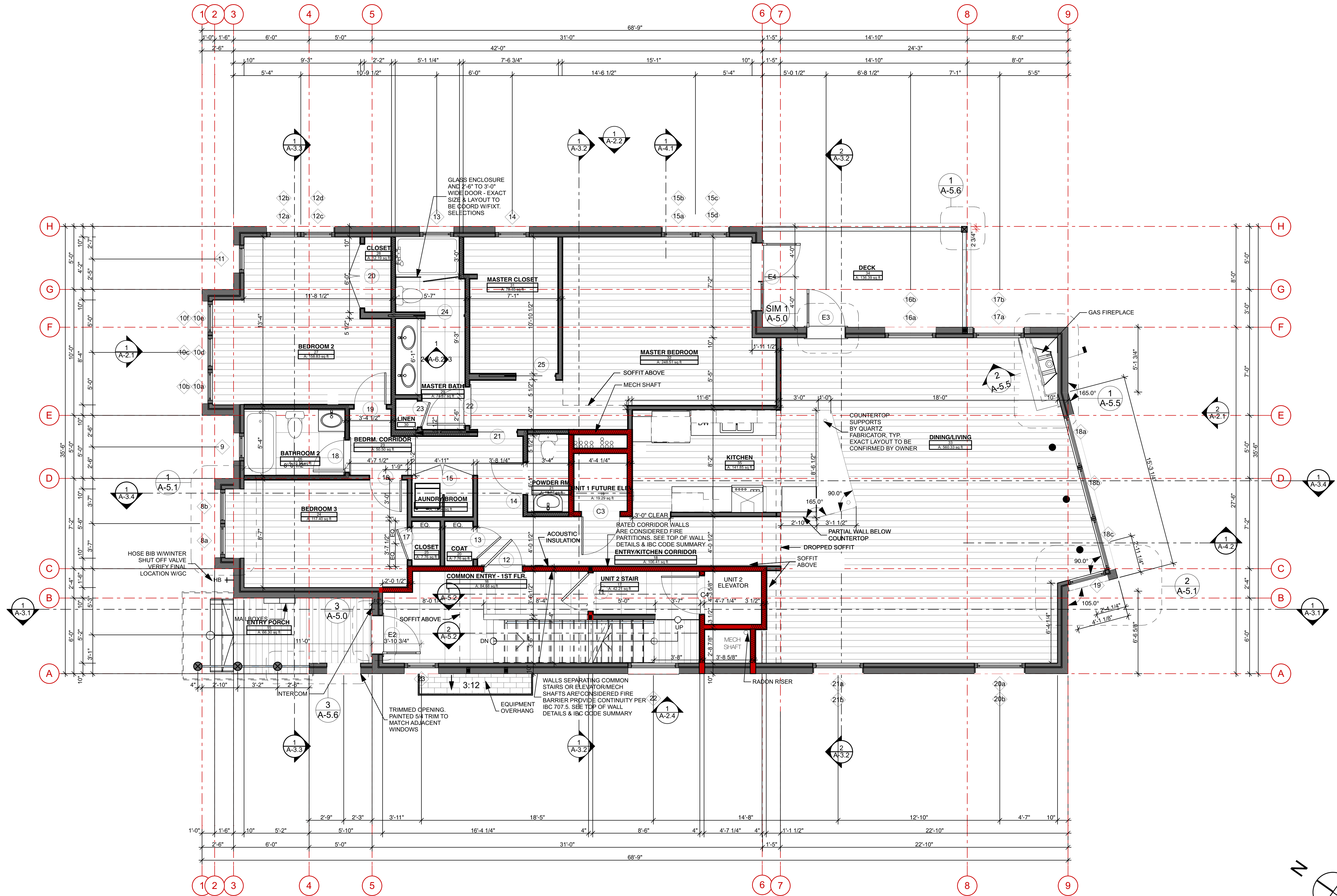
1 FIRST FLOOR SCALE: 1/4" = 1'-0"
