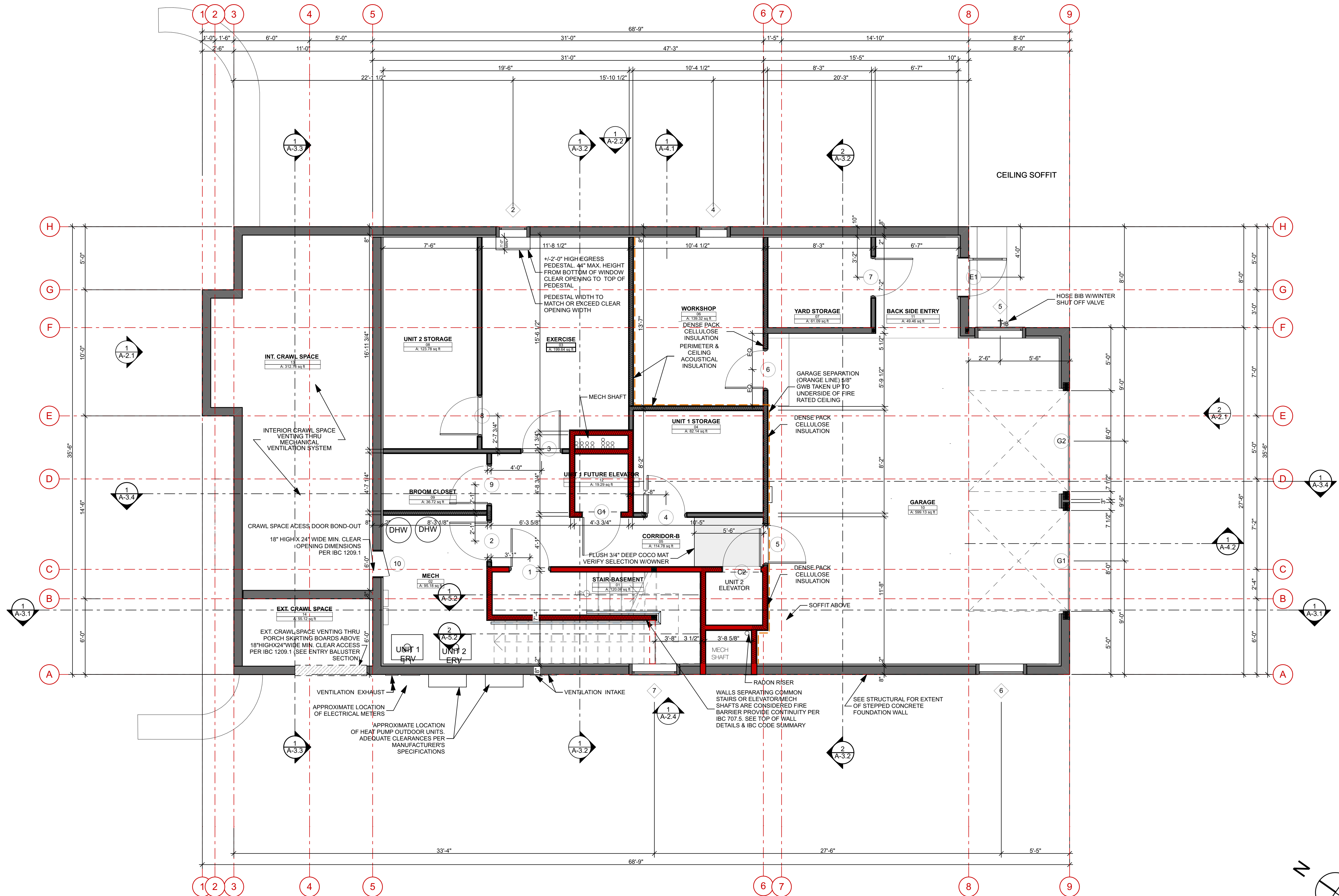
1 BASEMENT SCALE: 1/4" = 1'-0"
