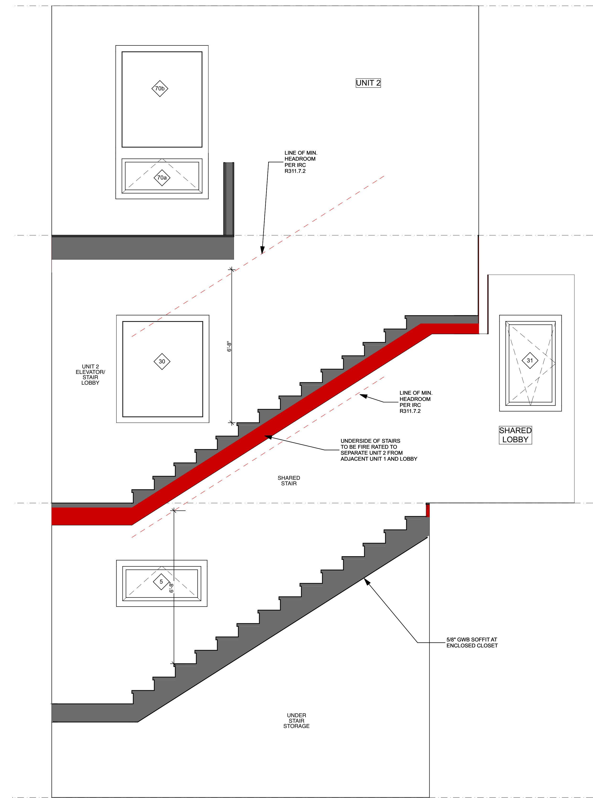
2 SECTION THRU STAIRS & ELEVATOR SCALE: 1/2" = 1'-0"
