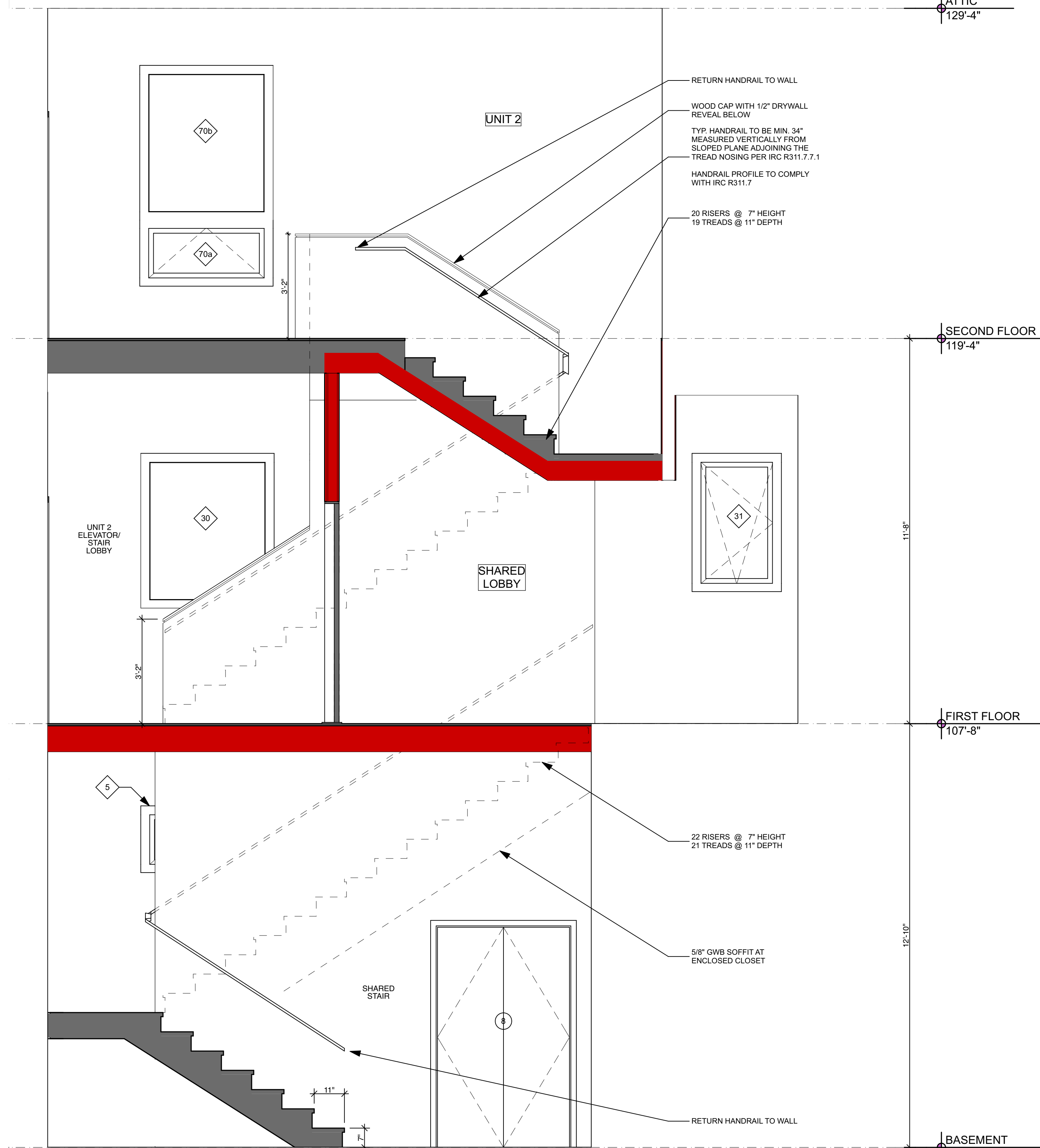
1 SECTION THRU STAIR & MECH CHASE SCALE: 1/2" = 1'-0"
