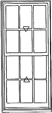
As Viewed From The Exterior Entered As: FS FS 33 1/4" X 73 3/8" RO 34 1/4" X 73 7/8"
