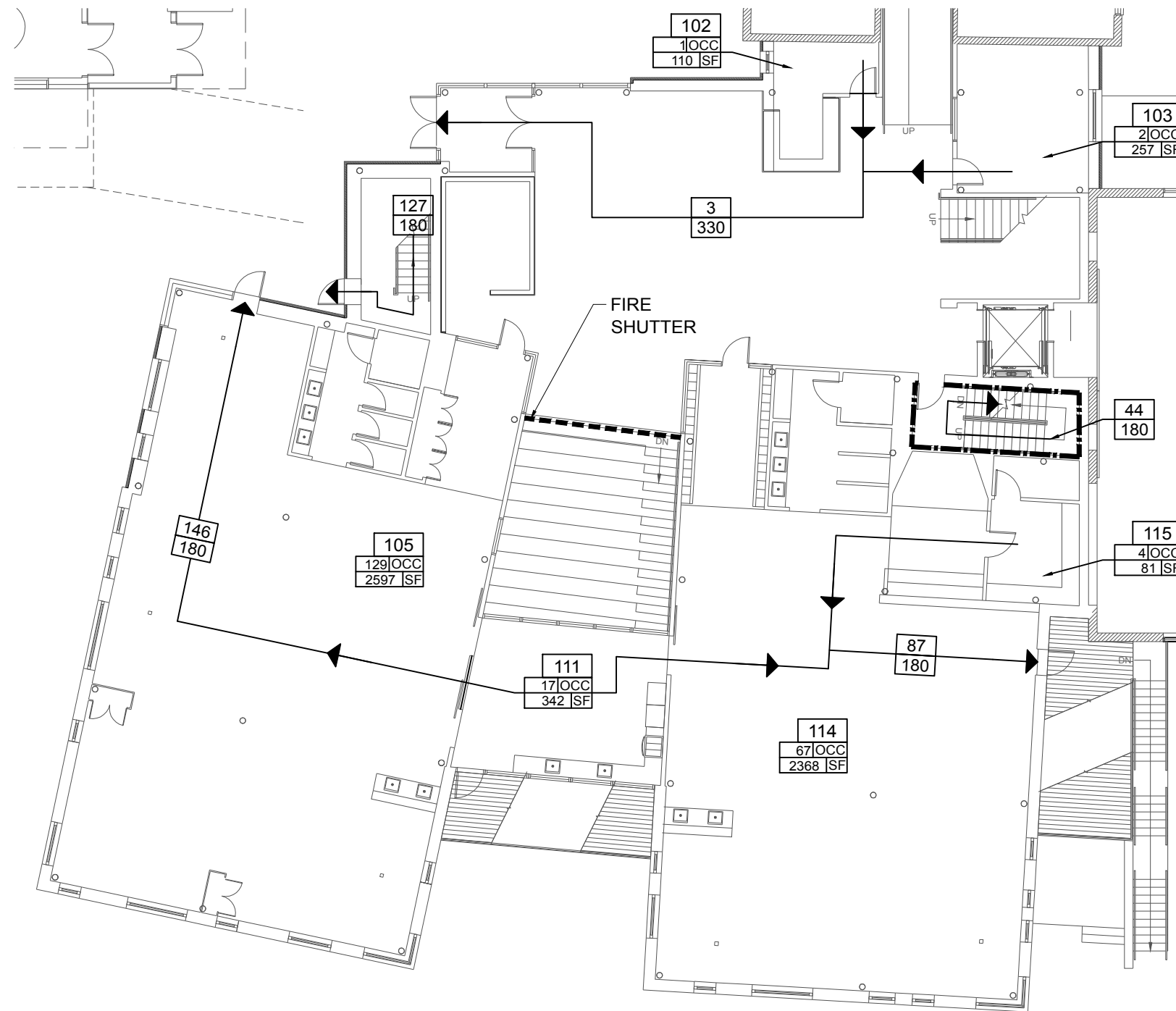
2 MAIN LEVEL LIFE SAFETY PLAN SCALE: 1/16" = 1'-0"
