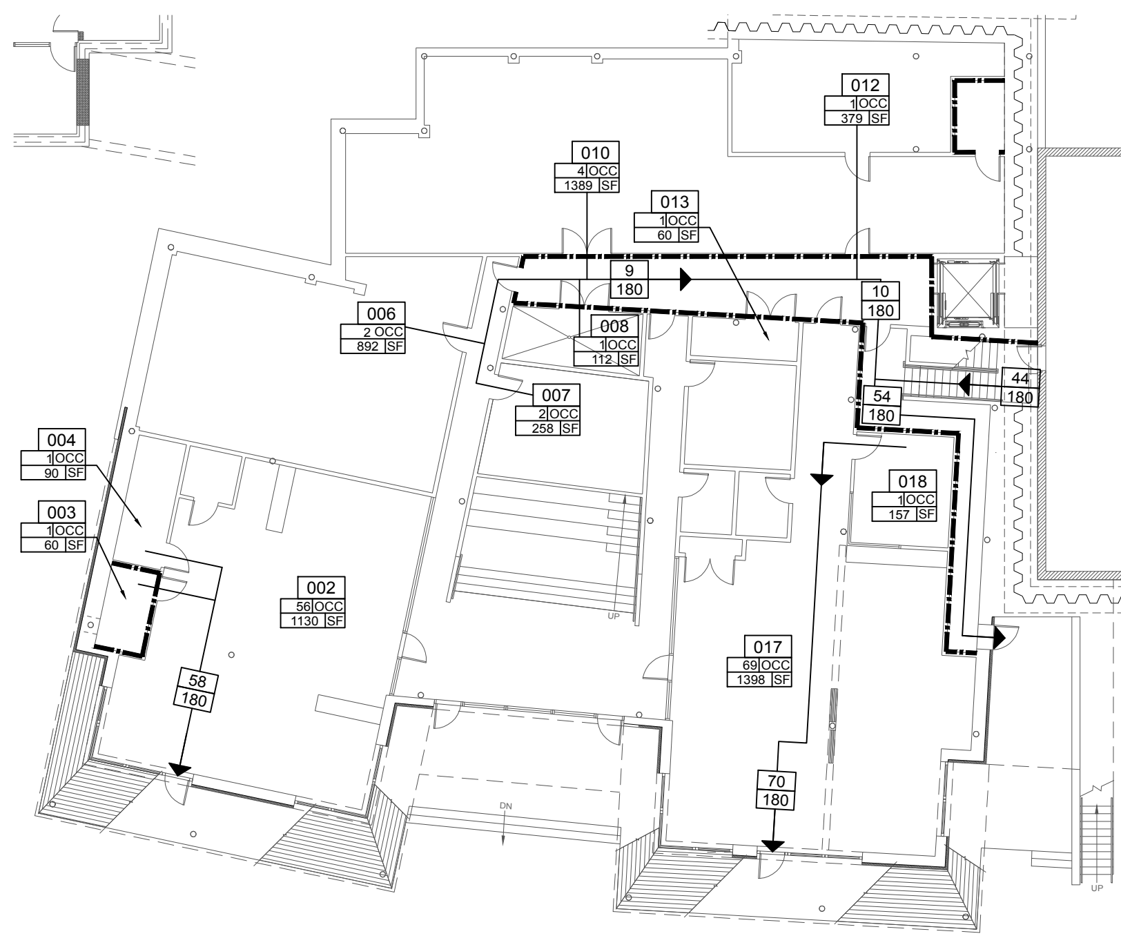
1 LOWER LEVEL LIFE SAFETY PLAN SCALE: 1/16" = 1'-0"
