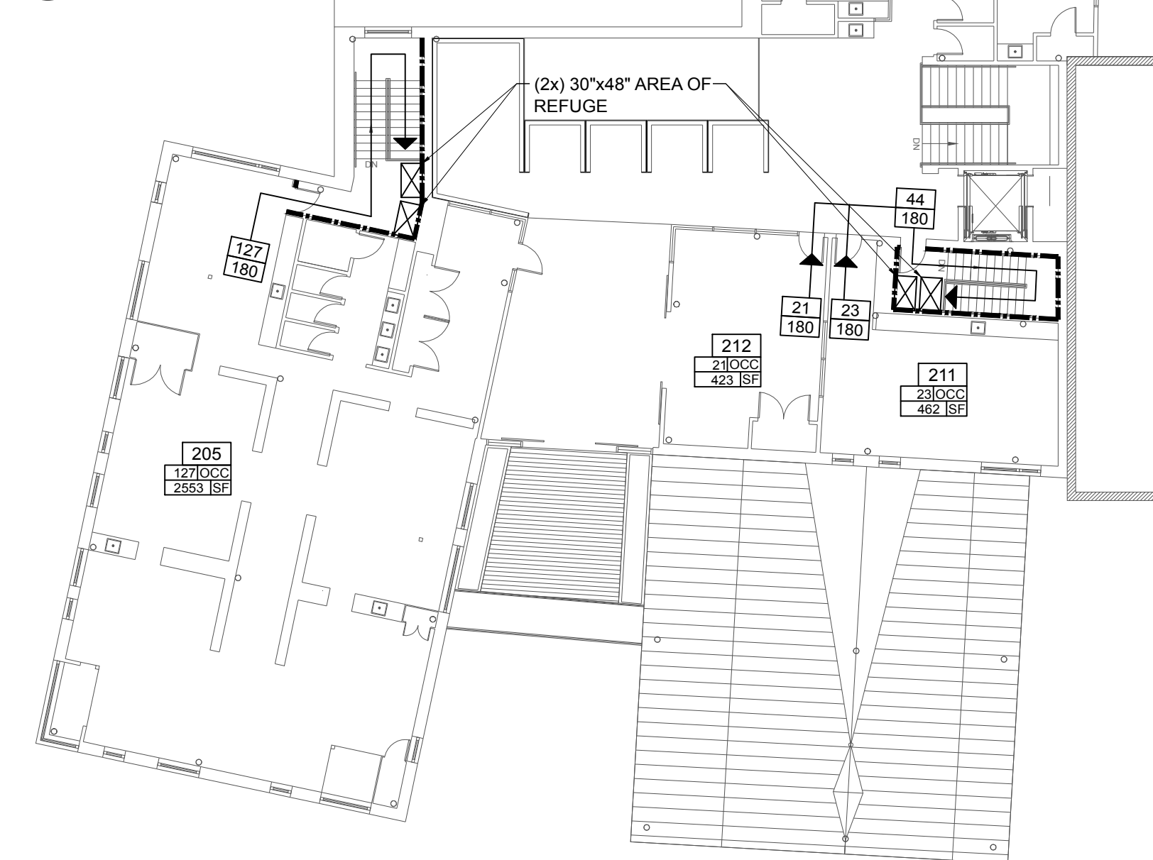
2 MAIN LEVEL LIFE SAFETY PLAN SCALE: 1/16" = 1'-0"
