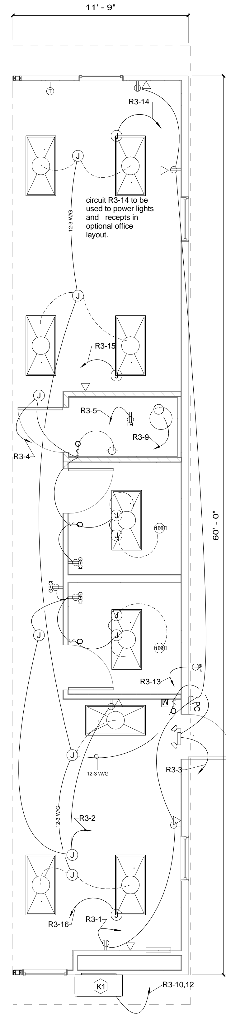
2 Electrical Plan 1/4" = 1'-0"
