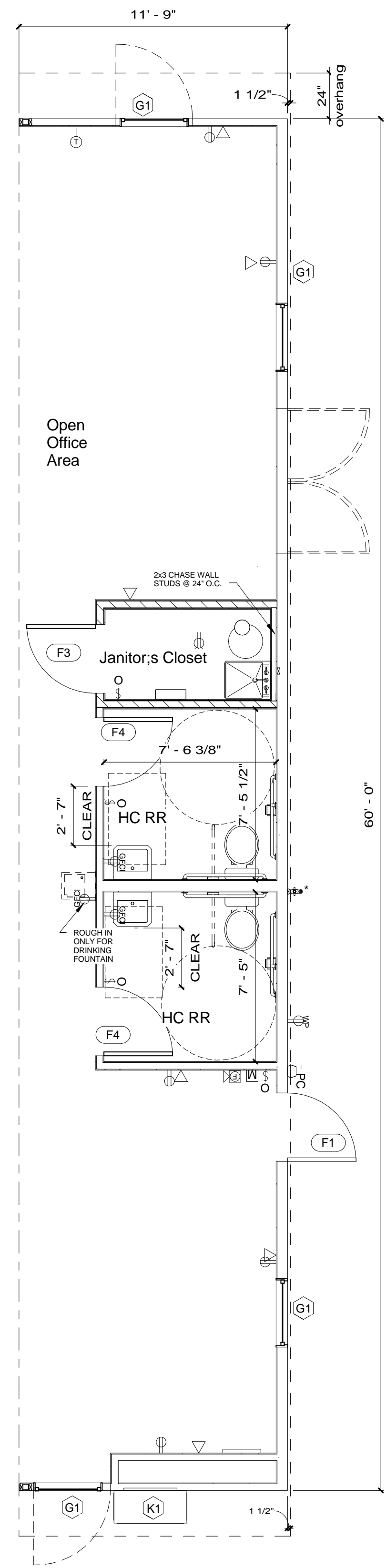
1 Floor Plan 1/4" = 1'-0"
