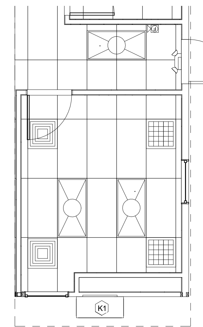
2a Ceiling Plan Office Opt 1 1/4" = 1'-0"
