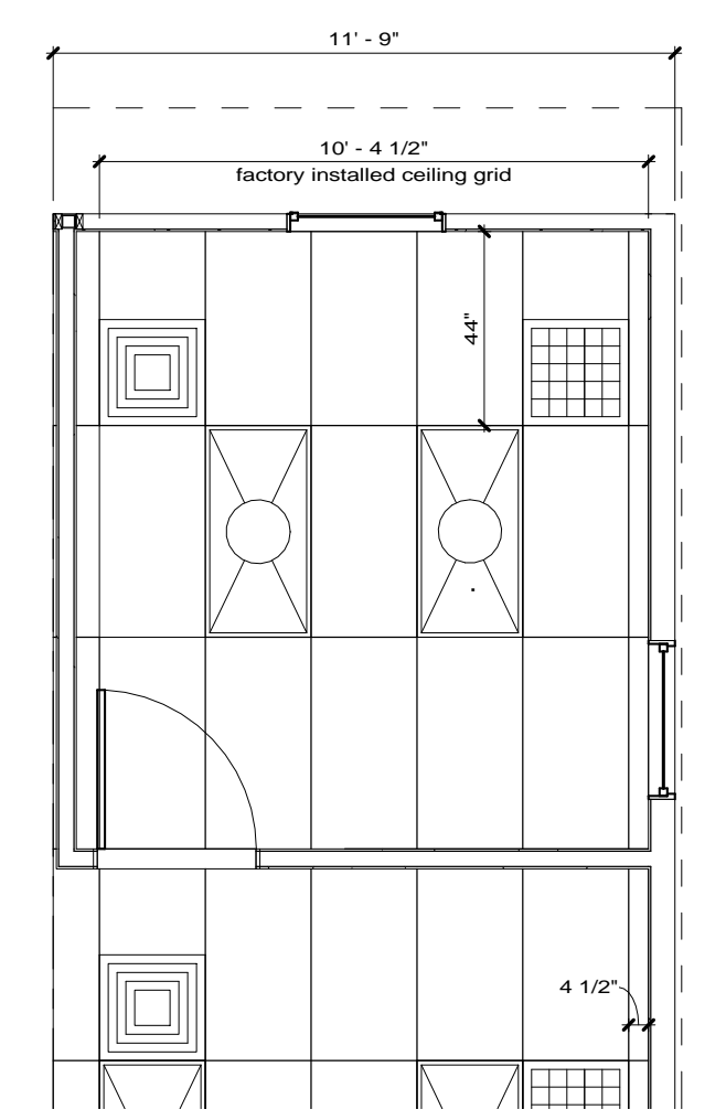
2b Ceiling Plan Office Opt 2 1/4" = 1'-0"
