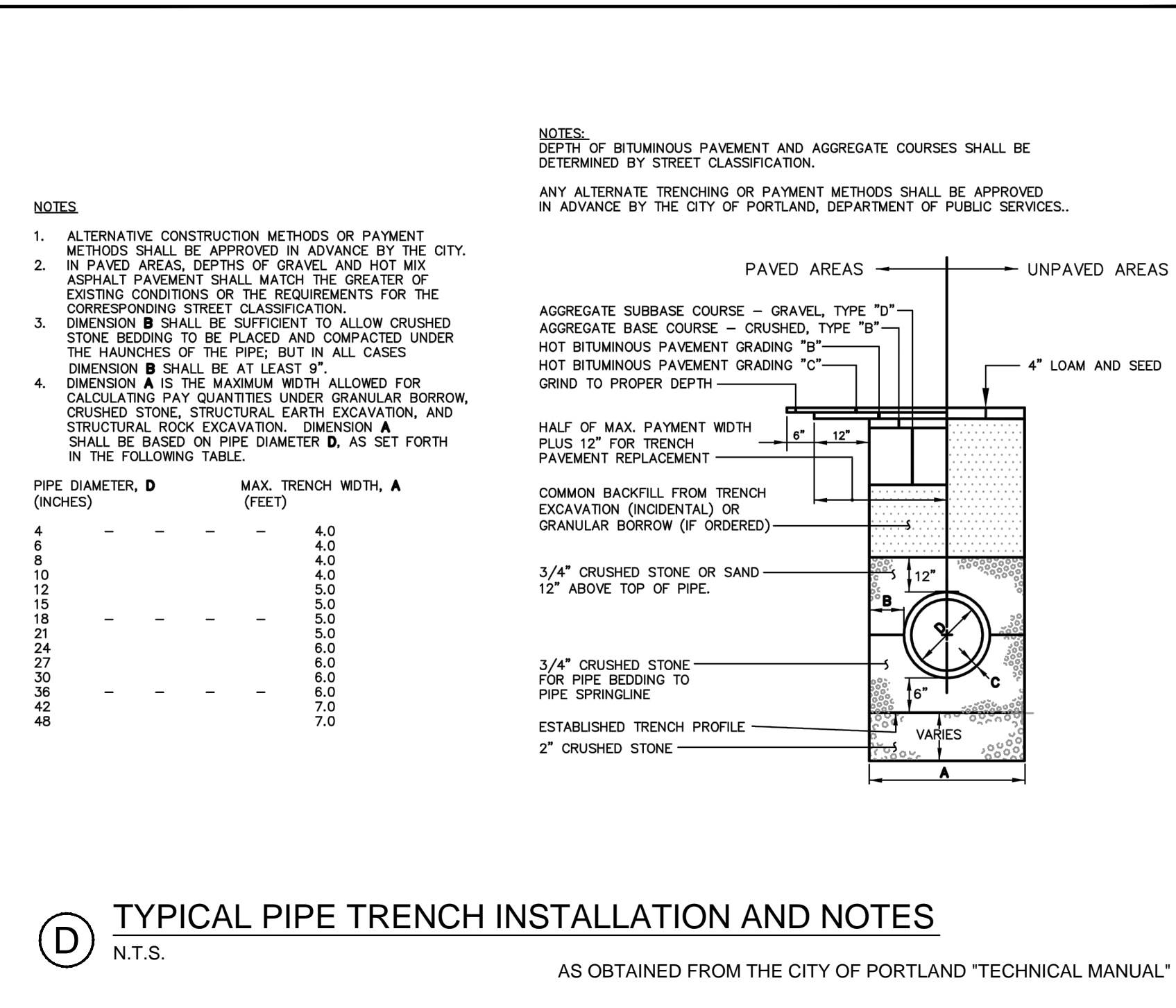
D TYPICAL PIPE TRENCH INSTALLATION AND NOTES N.T.S. AS OBTAINED FROM THE CITY OF PORTLAND "TECHNICAL MANUAL"
