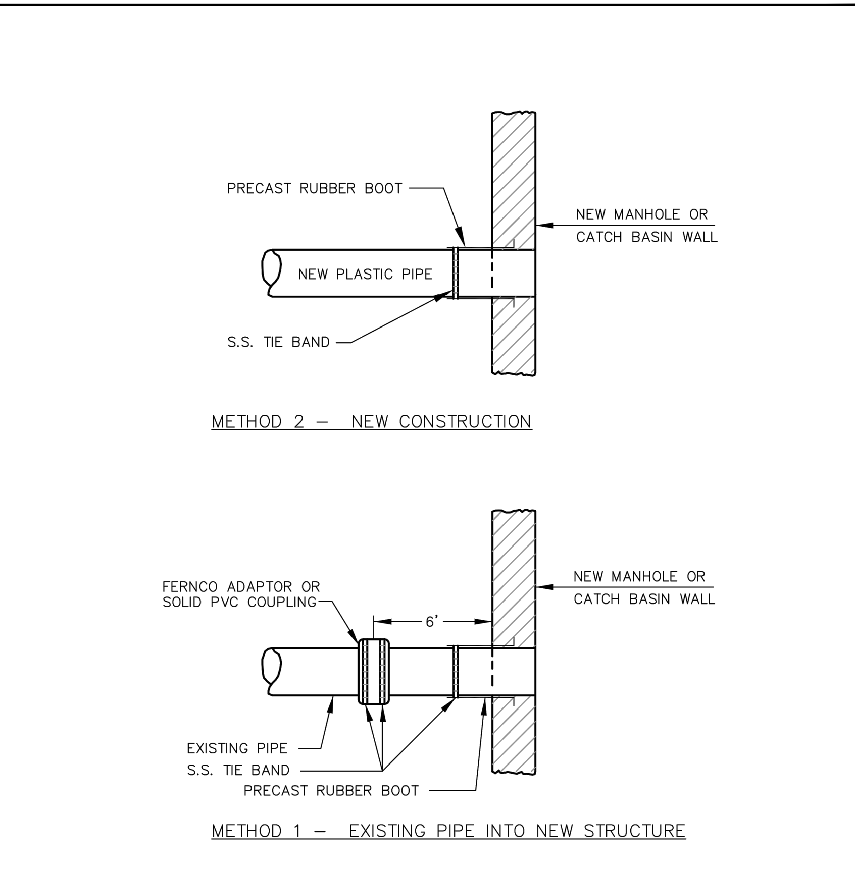
G PLASTIC PIPE CONNECTIONS NOT TO SCALE
