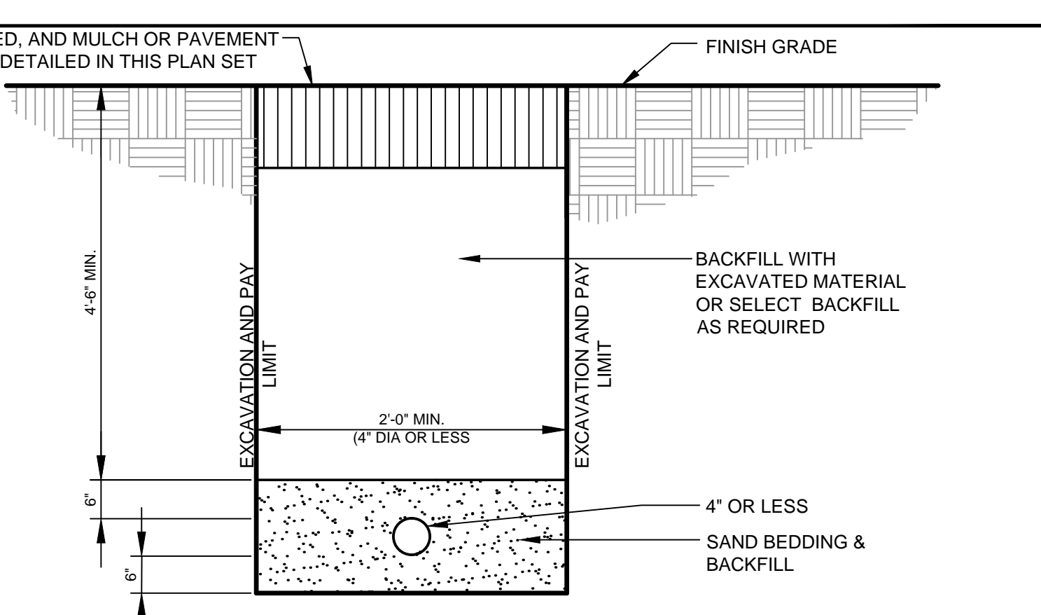
B WATER SERVICE TRENCH DETAIL N.T.S.
