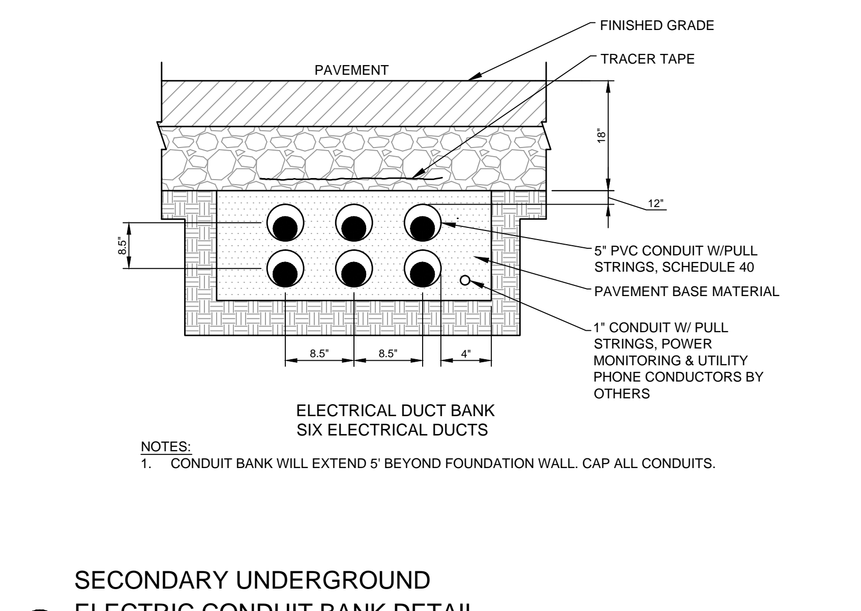
I SECONDARY UNDERGROUND ELECTRIC CONDUIT BANK DETAIL N.T.S.
