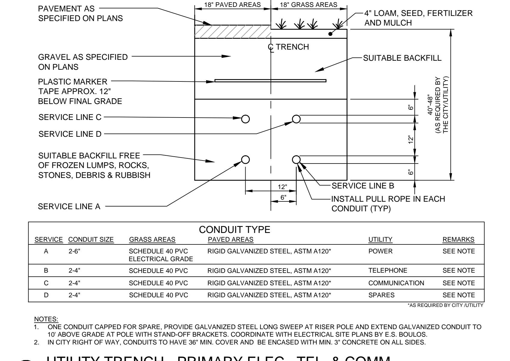
F UTILITY TRENCH - PRIMARY ELEC., TEL. & COMM. N.T.S.
