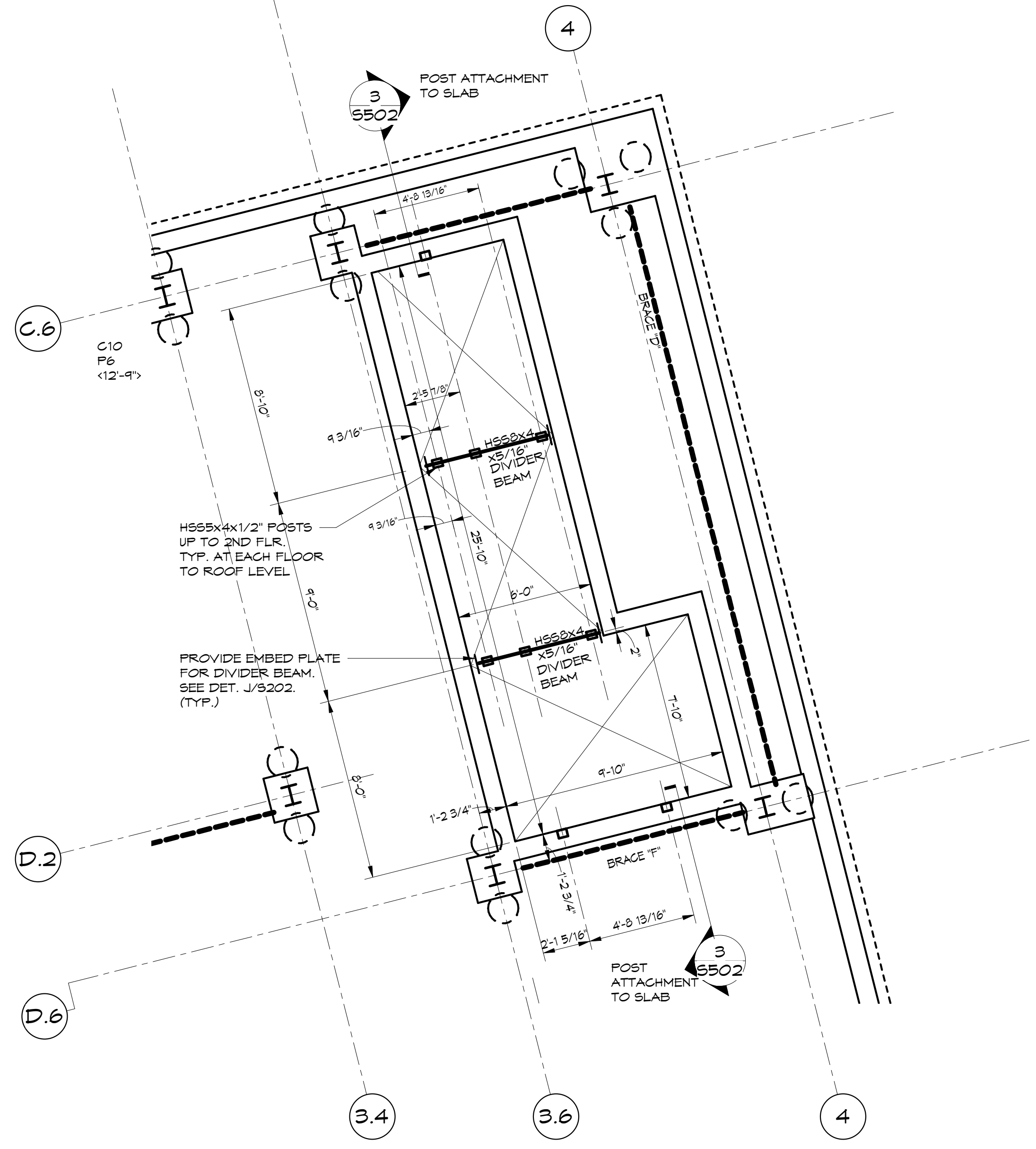
1 ELEVATOR POSTS PART PLAN 1/4" = 1'-0"
