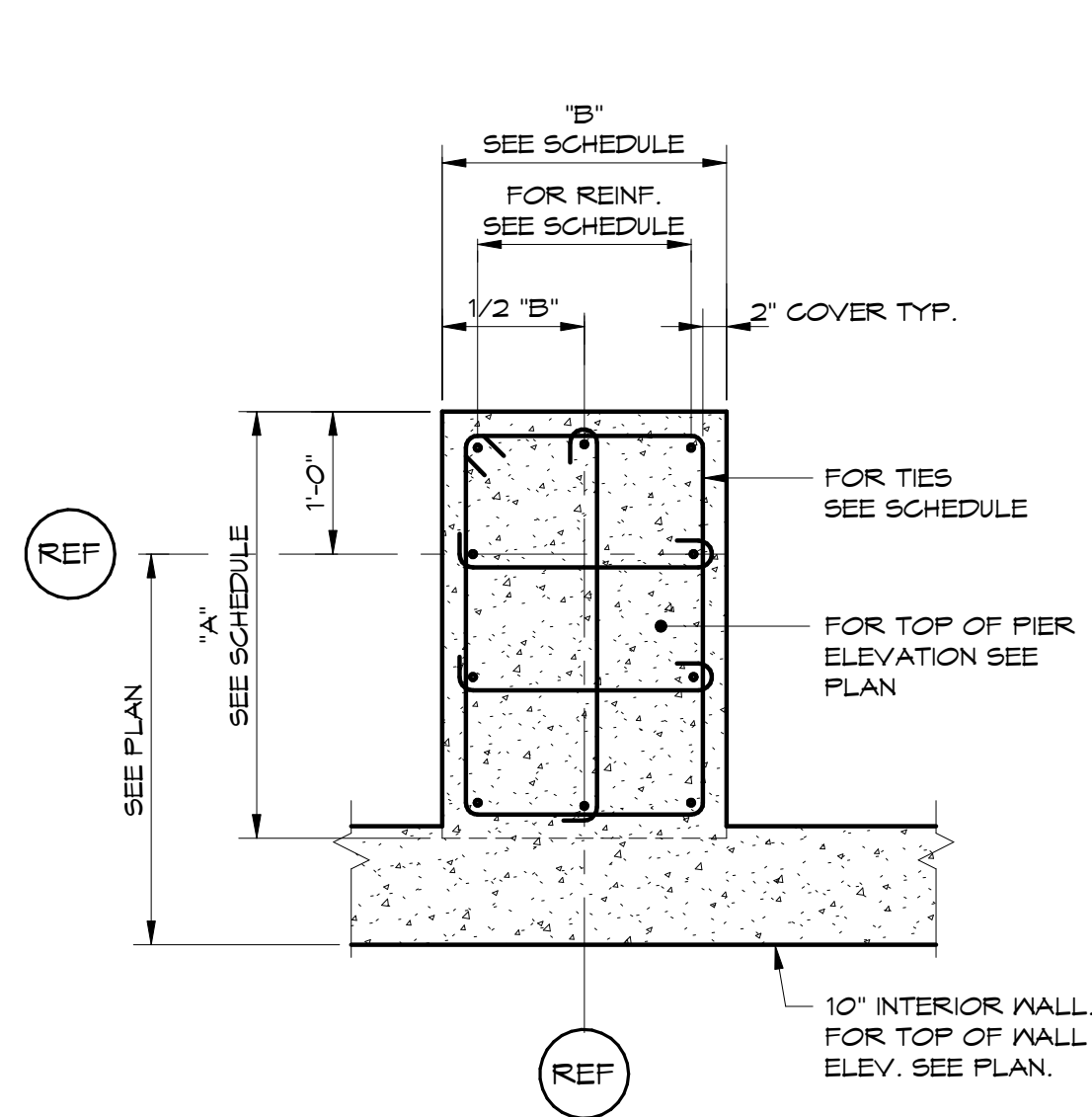
PIER DETAIL - TYPE E
