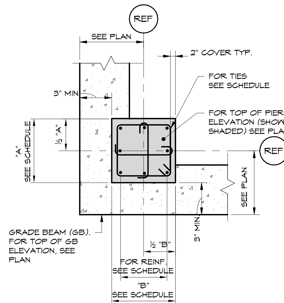
PIER DETAIL - TYPE C
