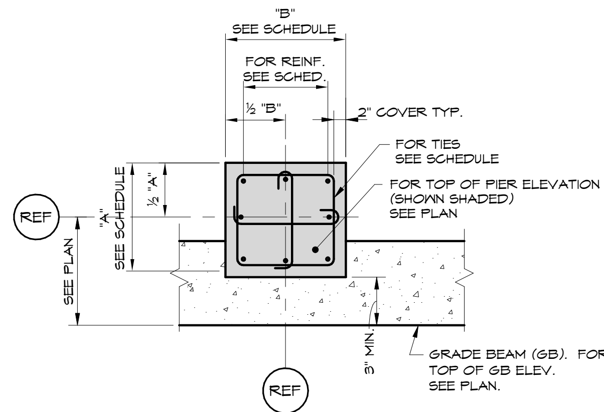
PIER DETAIL - TYPE B
