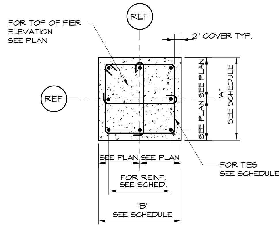
PIER DETAIL - TYPE A
