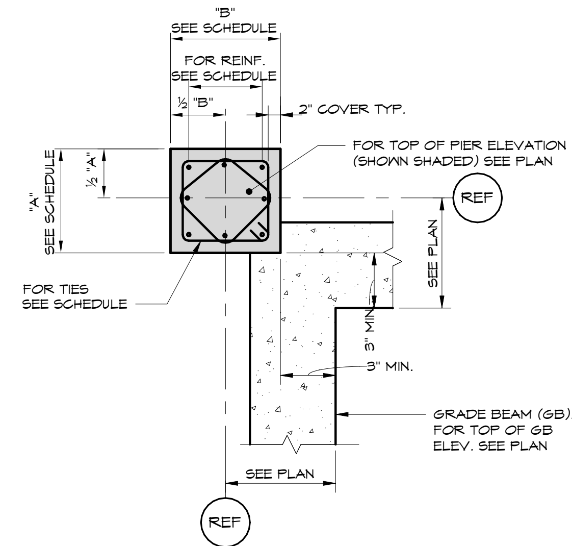
PIER DETAIL - TYPE D
