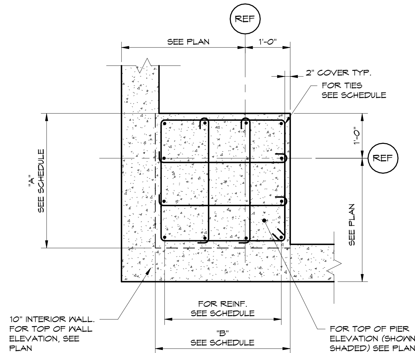
PIER DETAIL - TYPE F
