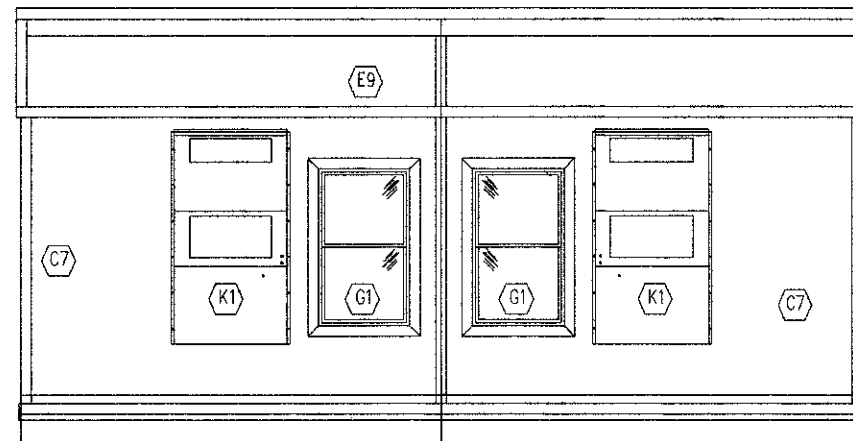
HITCH ENDWALL ELEVATION
