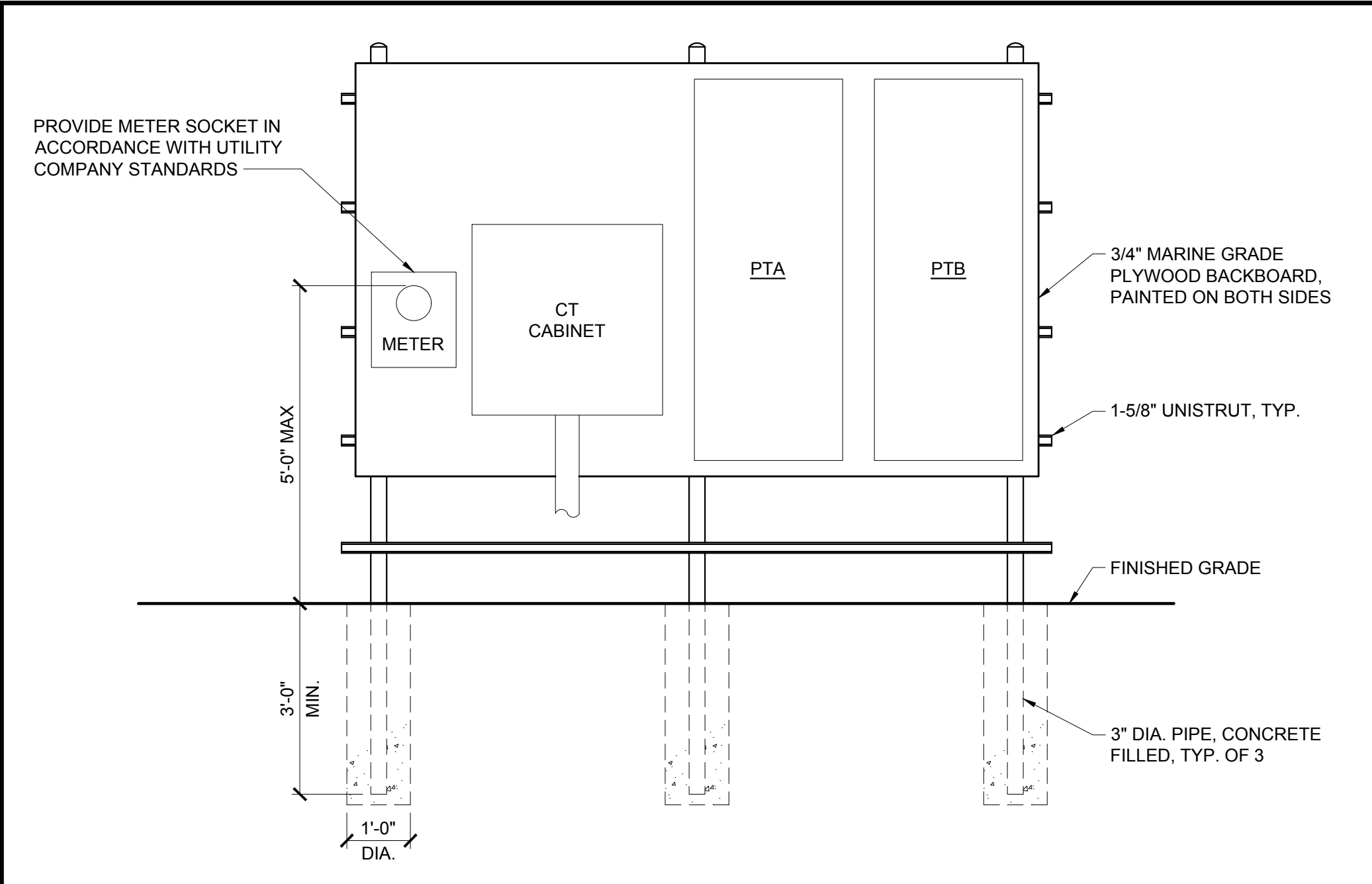
A3 BACKBOARD DETAIL NO SCALE
