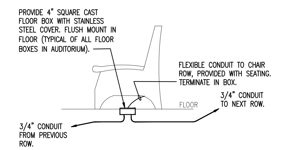
AUDITORIUM SEATING DETAIL N.T.S.
