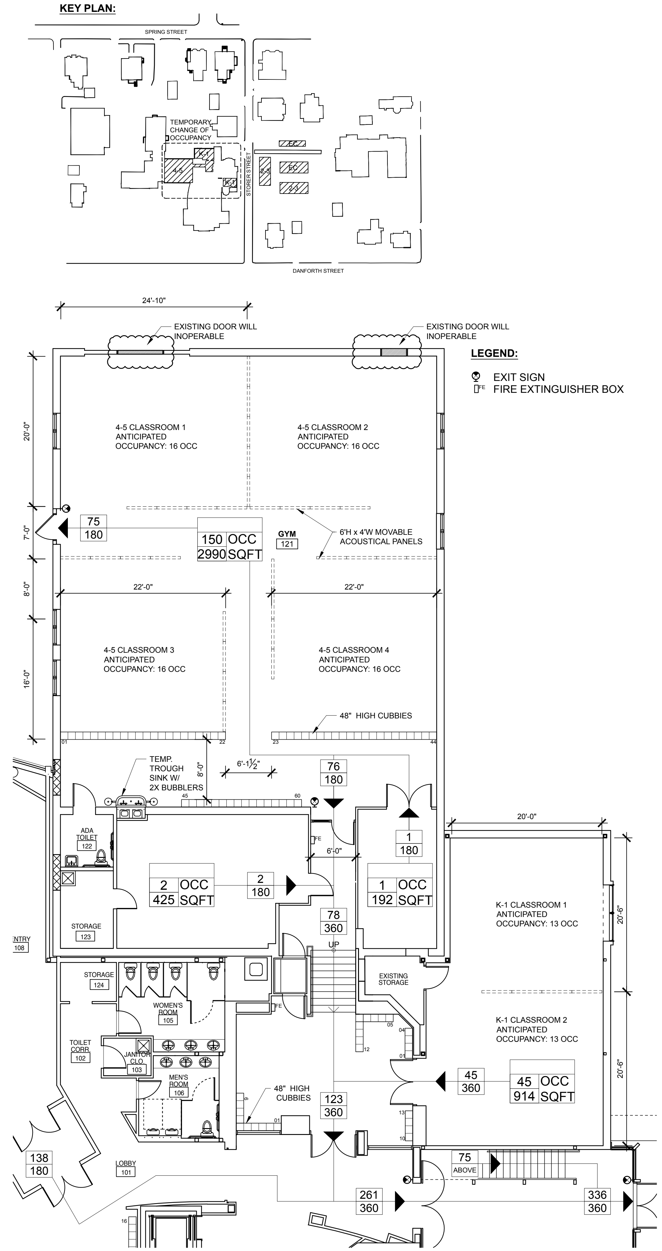
1 FIRST FLOOR PLAN - GYM AND GALLERY SCALE: 1/8" = 1'-0"
