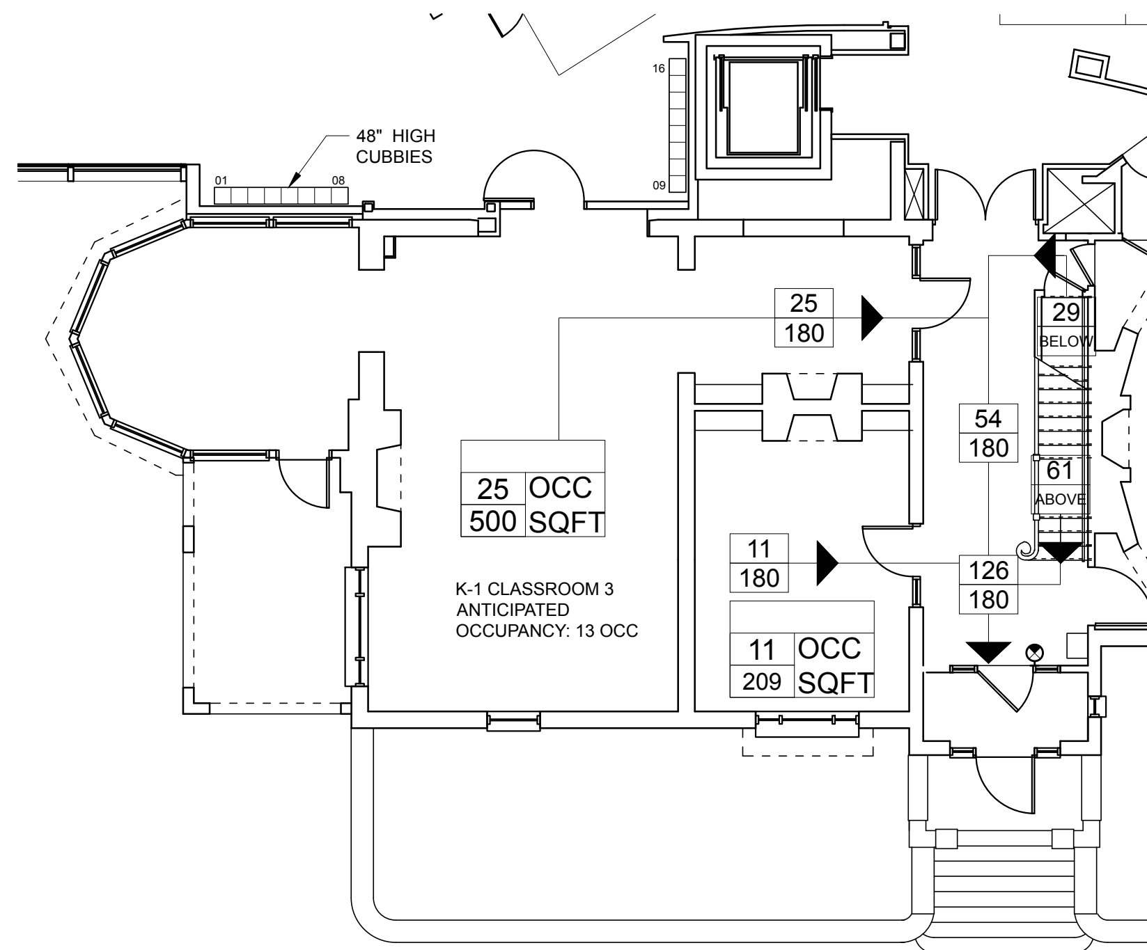
2 FIRST FLOOR PLAN - MUSIC ROOM SCALE: 1/8" = 1'-0"
