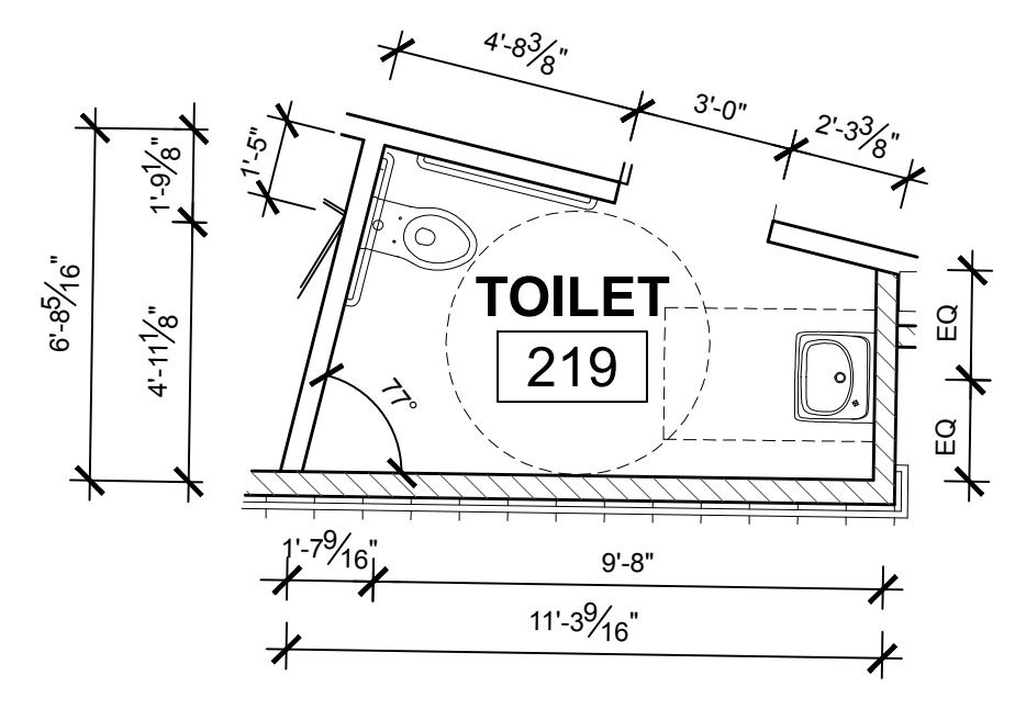
3 UPPER LEVEL FLOOR PLAN - TLT SCALE: 1/4" = 1'-0"
