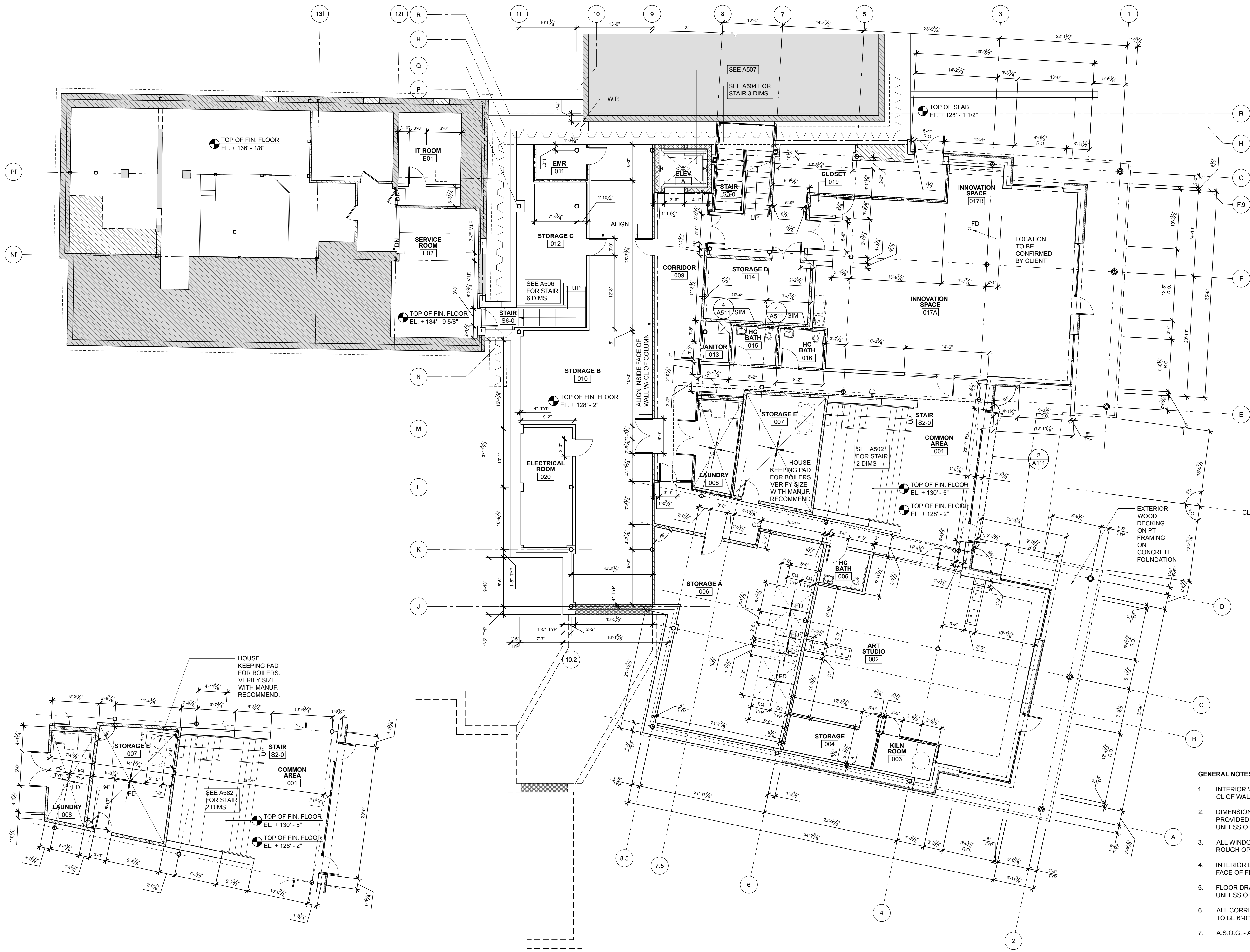
2 LOWER LEVEL FLOOR PLAN - COMMON AREA SCALE: 1/8" = 1'-0"
