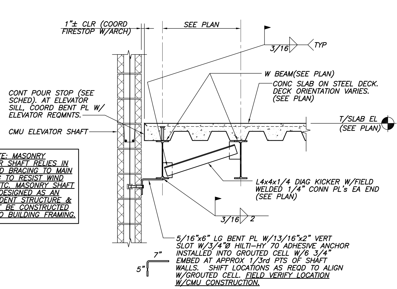
TYP ELEVATOR SHAFTWALL BRACING DETAIL N.T.S.
