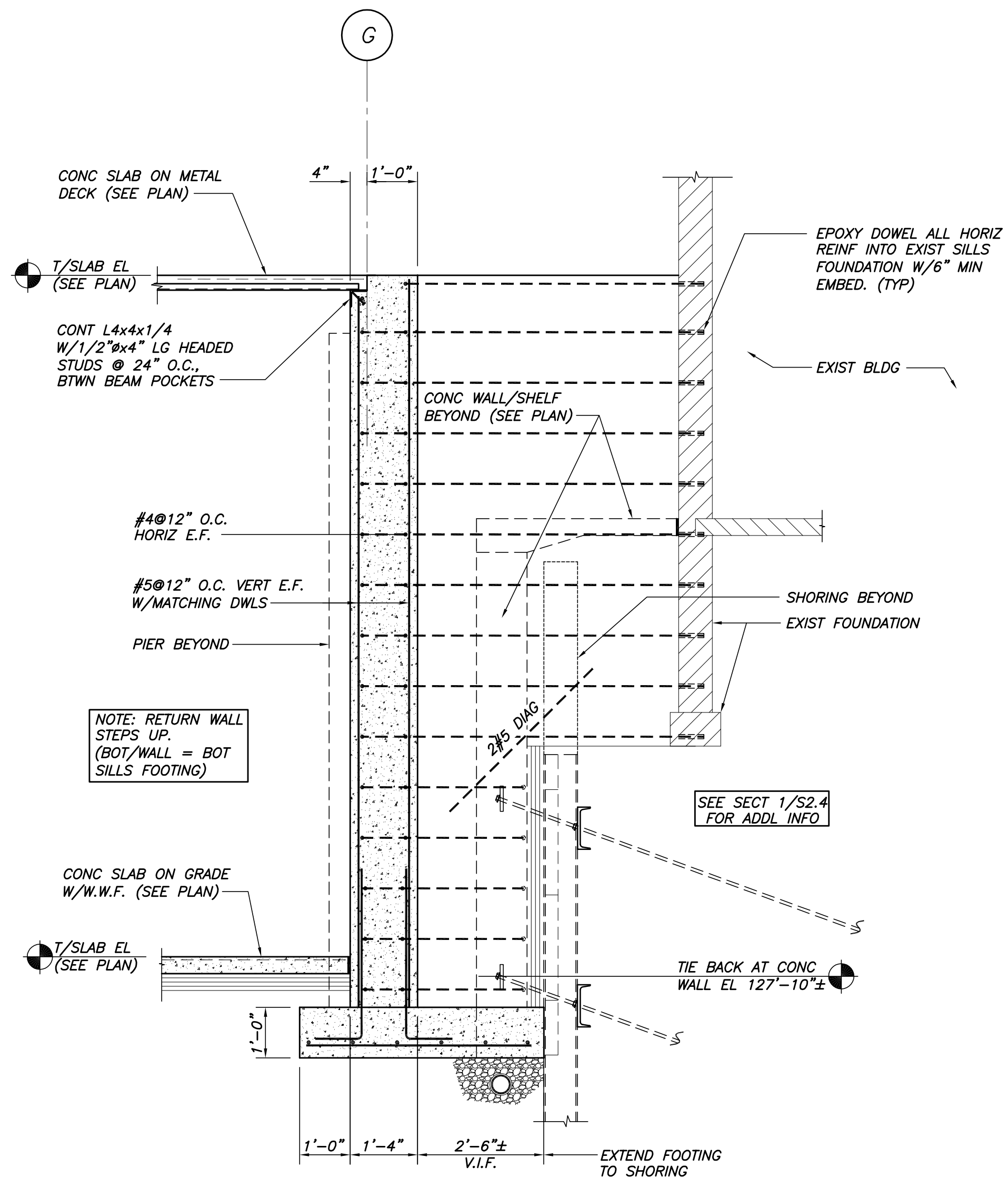
SECTION 1 1/2"=1'-0"
