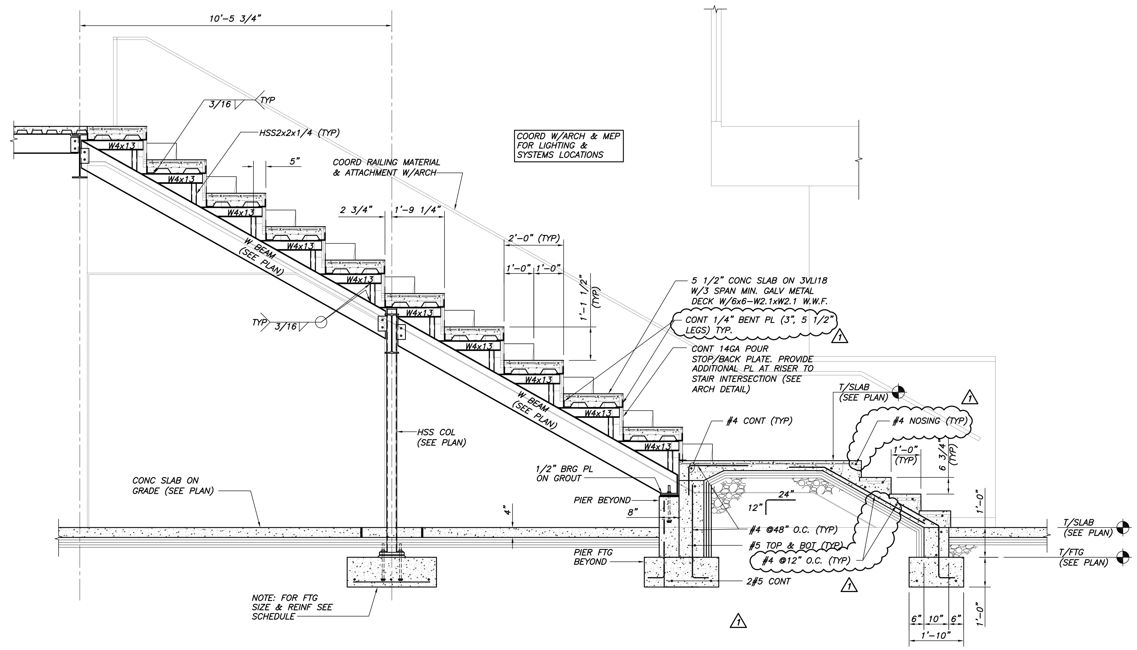
SECTION 2 1/2"=1'-0"
