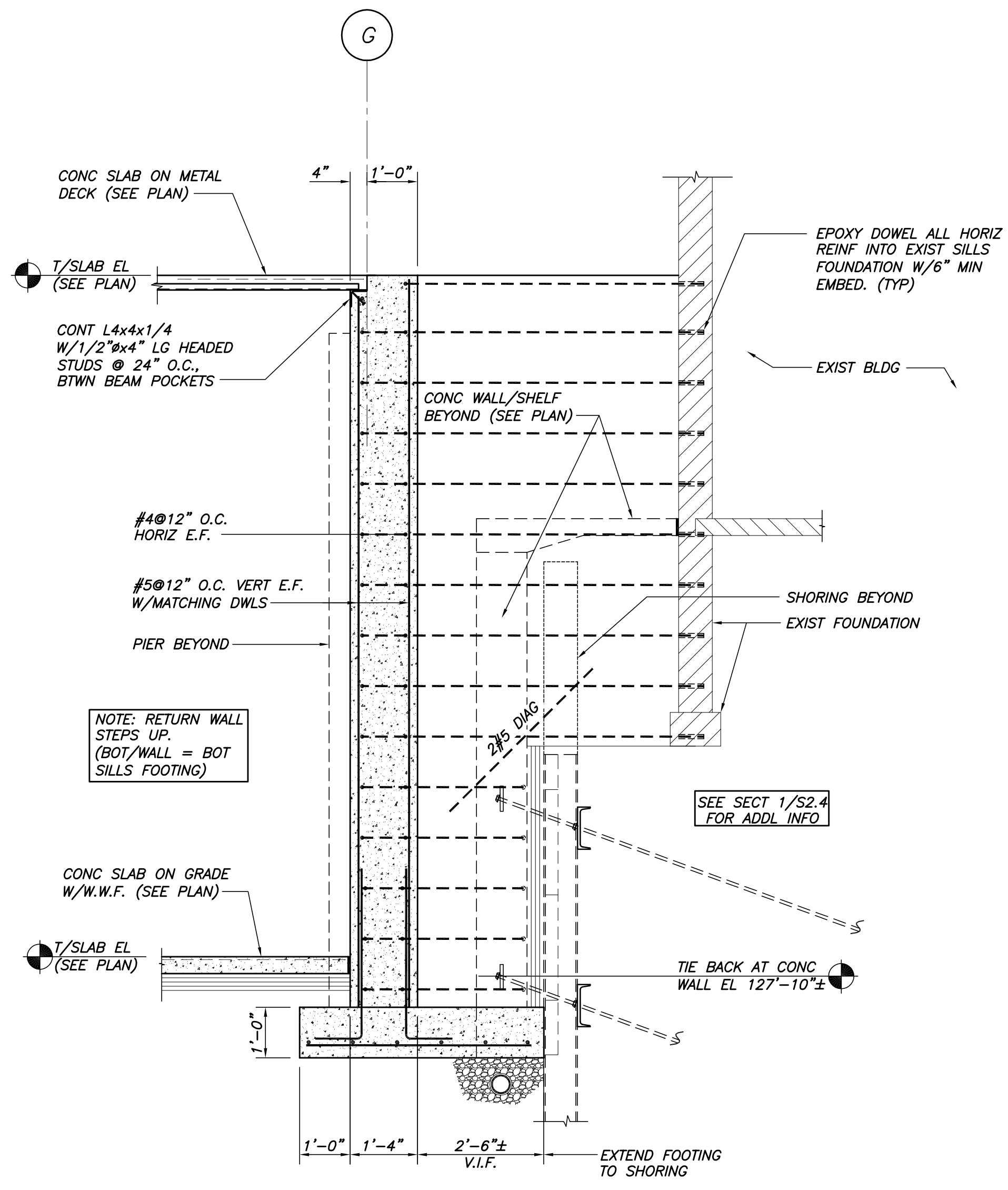
SECTION 1 1/2"=1'-0"
