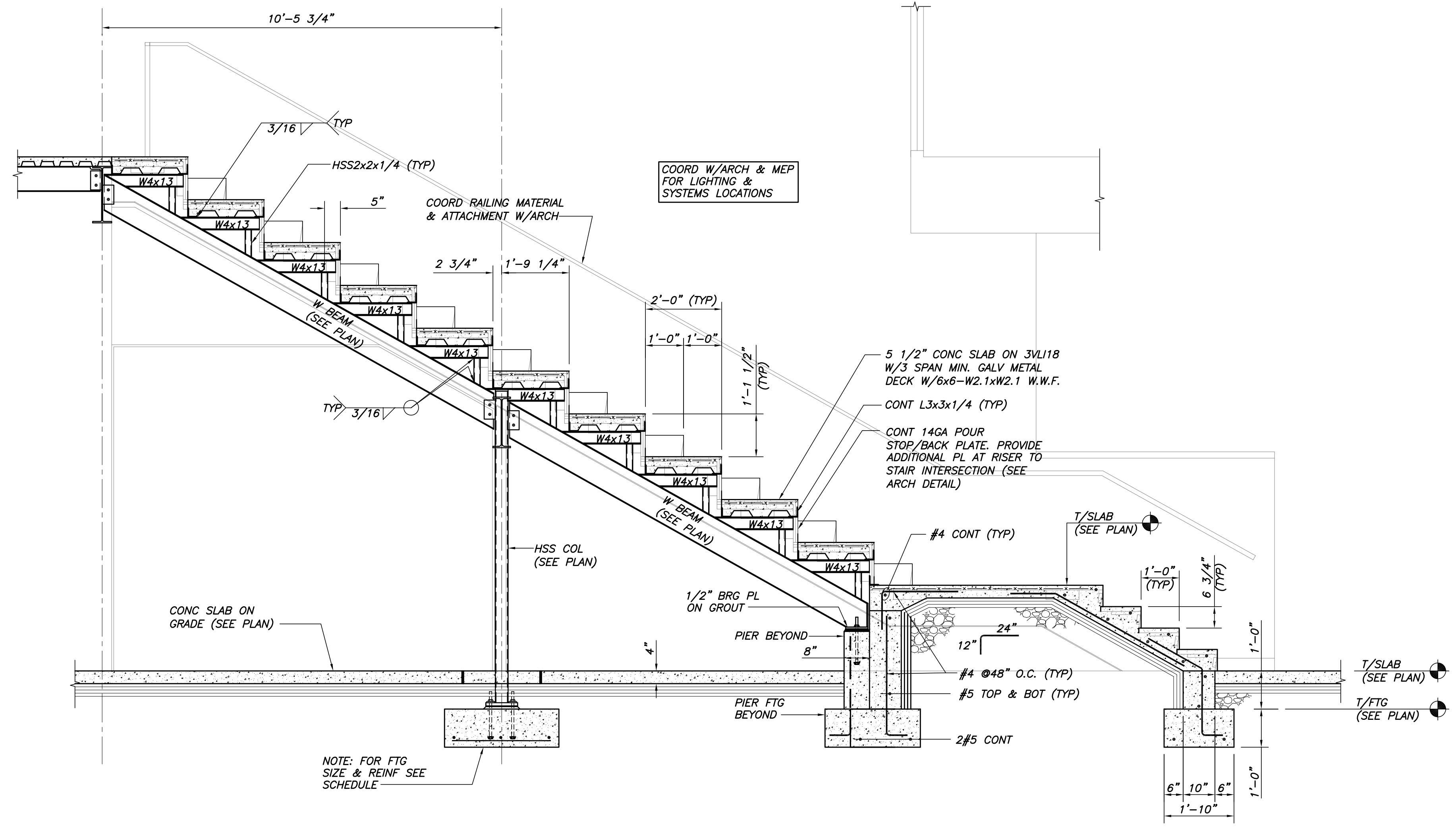
SECTION 2 1/2"=1'-0"
