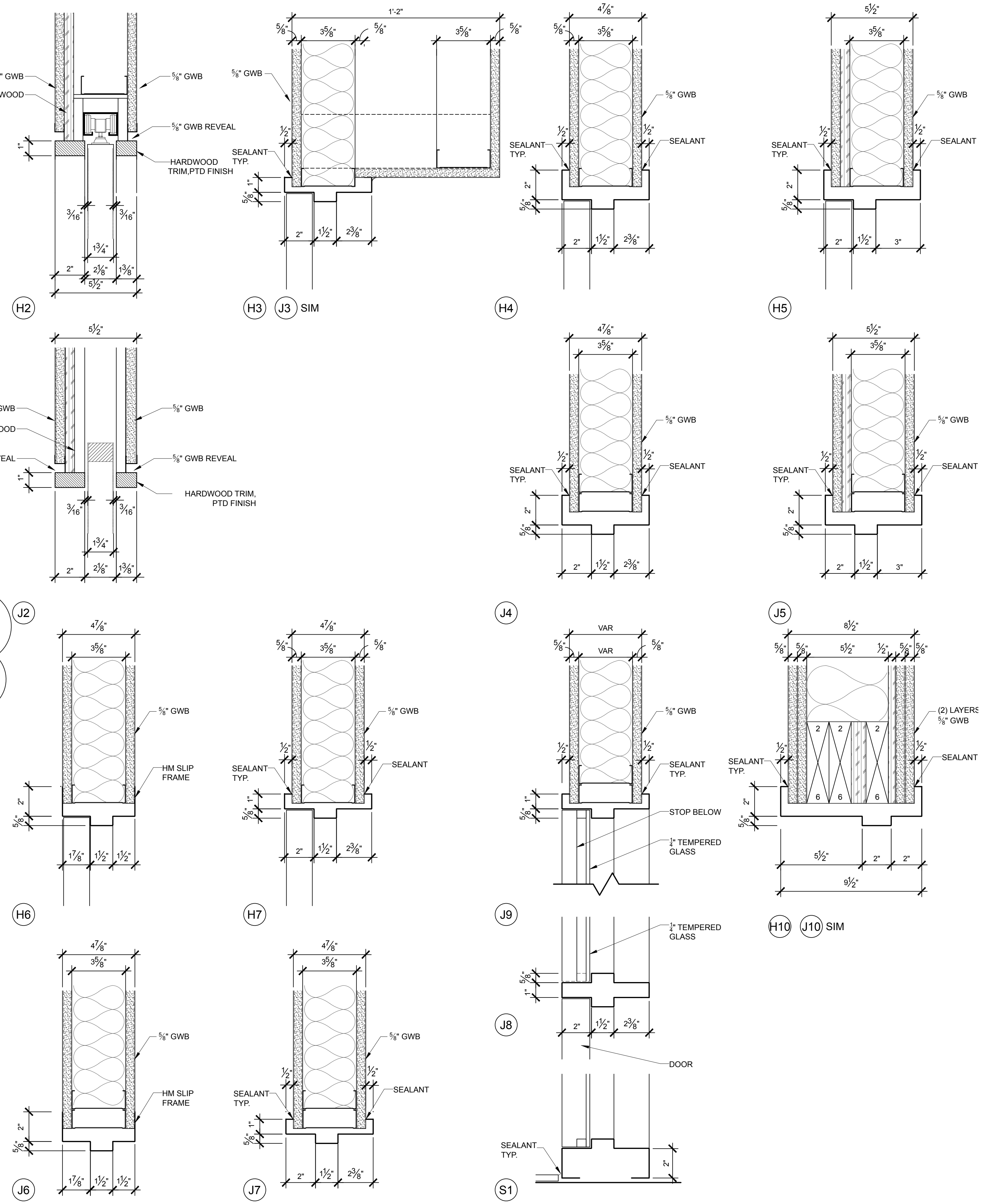
1 DOOR HEADER AND JAMB DETAILS SCALE: 3" = 1'-0"
