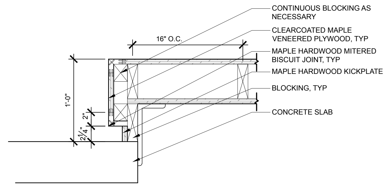
1 PLATFORM AT LOBBY ROOM 101 SCALE: 1 1/2" = 1'-0"
