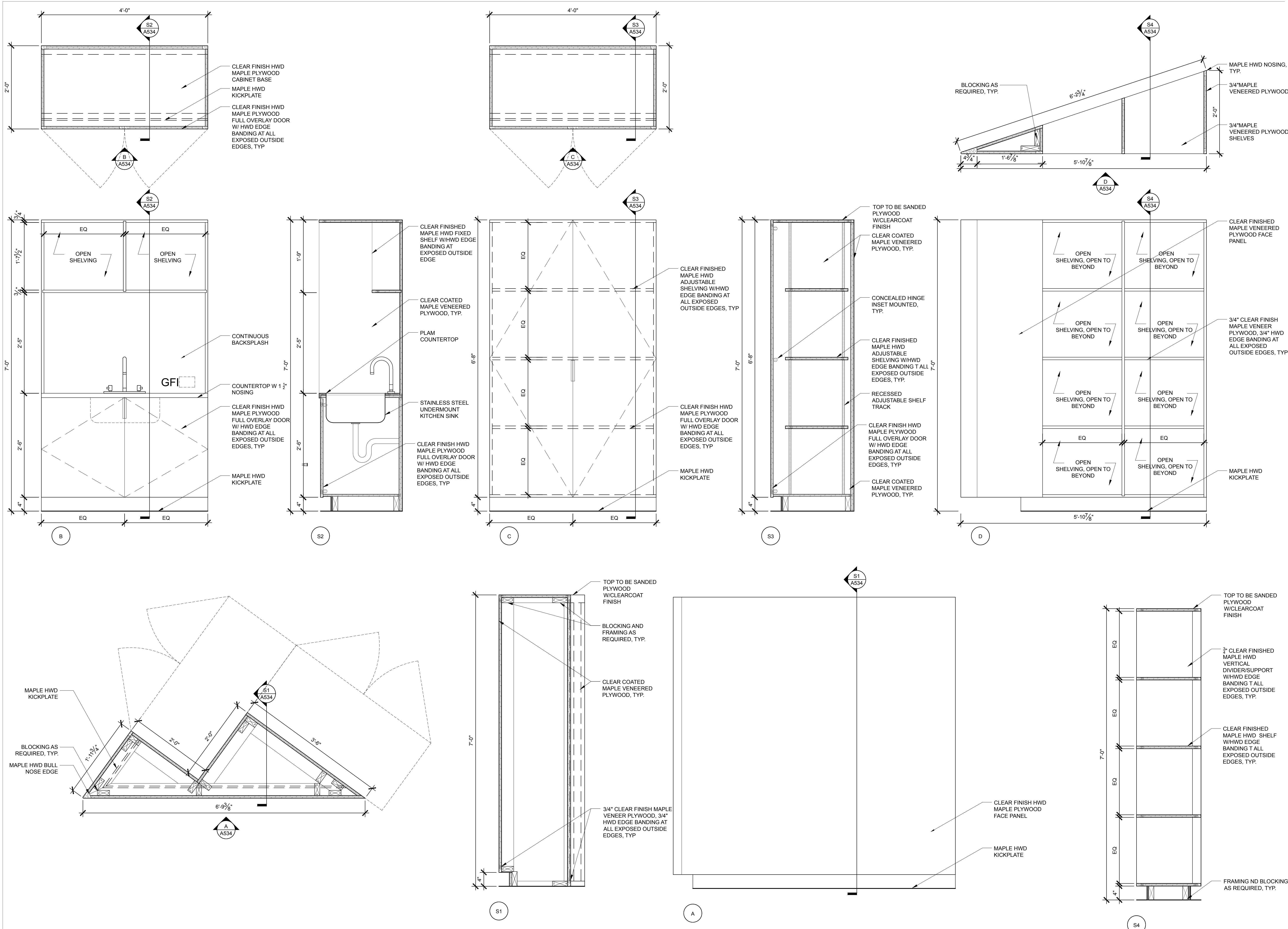
1 4-5 CLASSROOM MILLWORK PLANS, SECTIONS, & ELEVATIONS SCALE: 1" = 1'-0"
