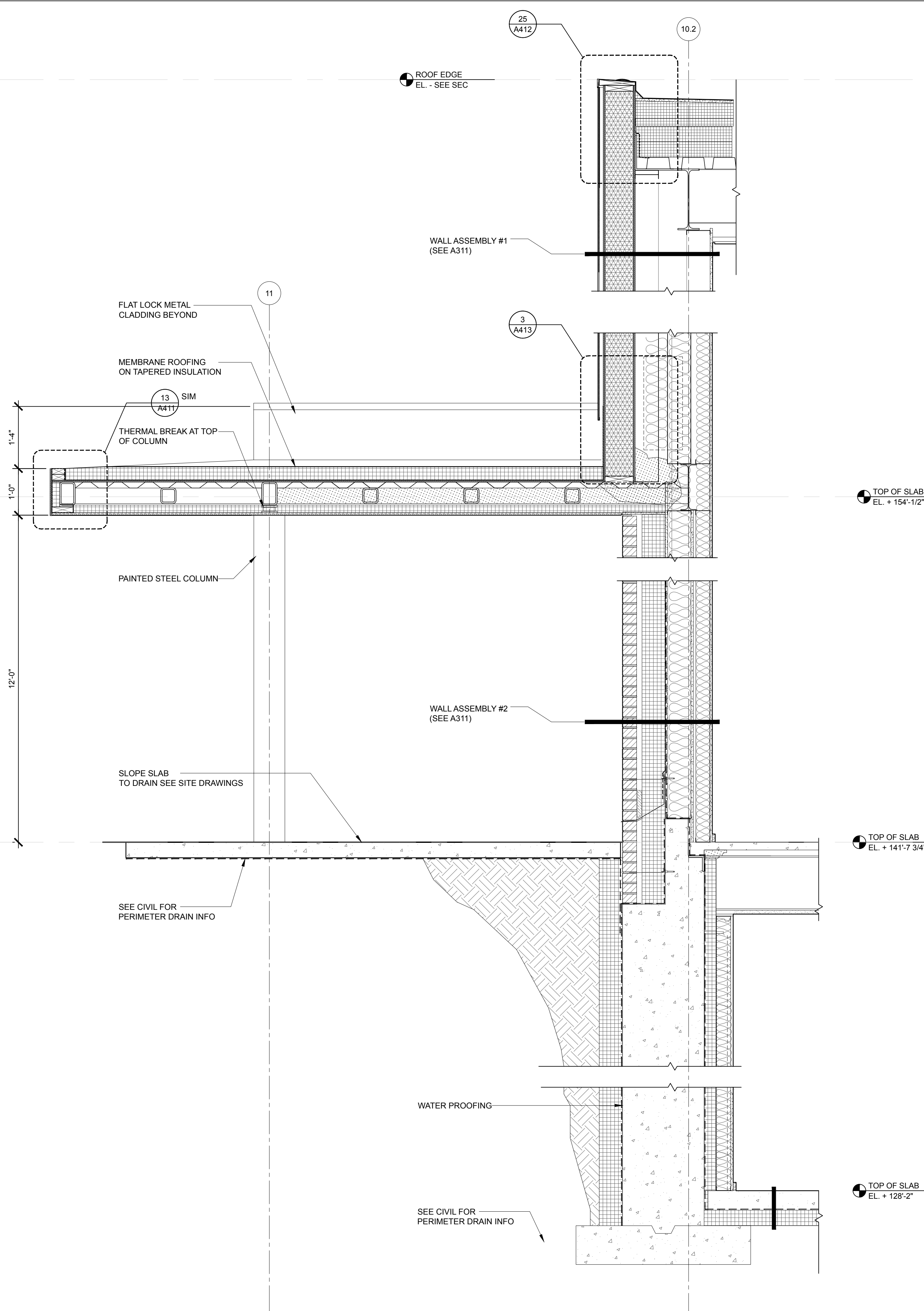
6 WALL SECTION, TYPICAL SCALE: 3/4" = 1'-0"
