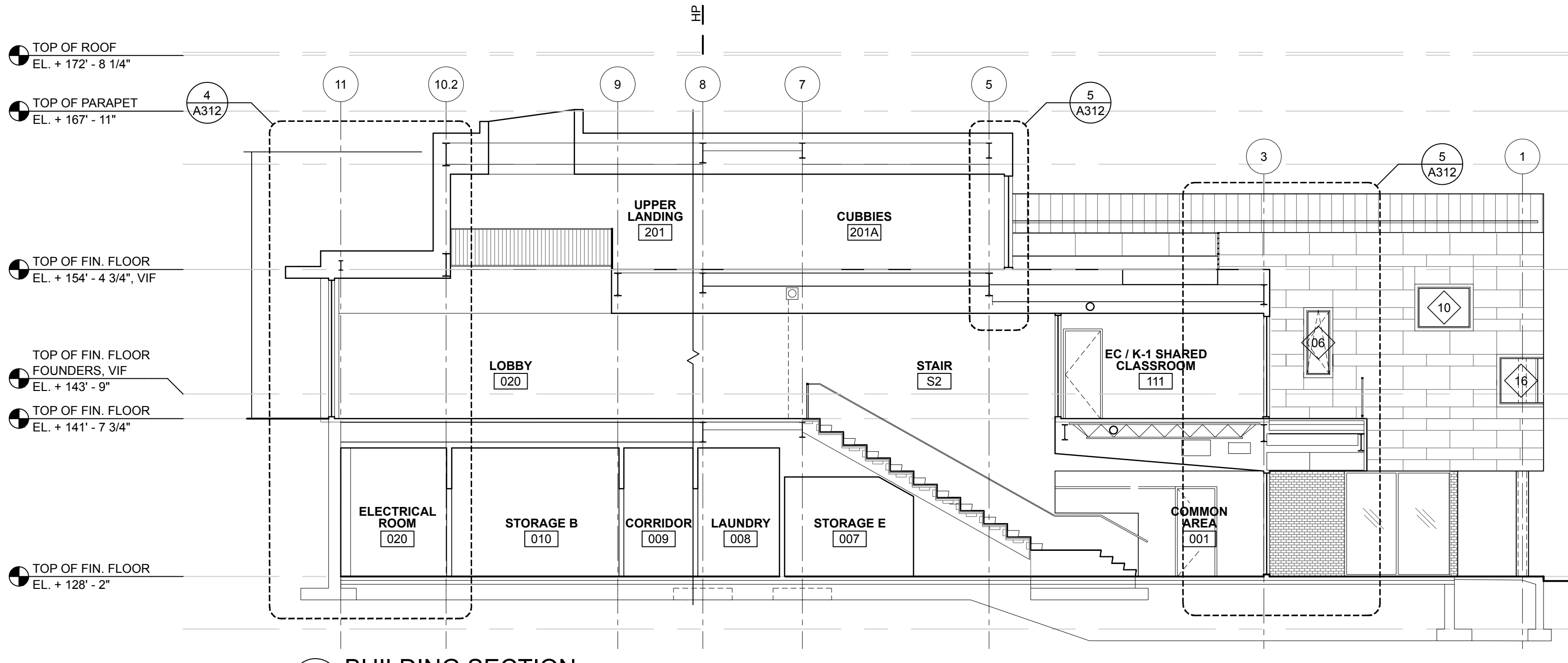
2 BUILDING SECTION SCALE: 1/8" = 1'-0"
