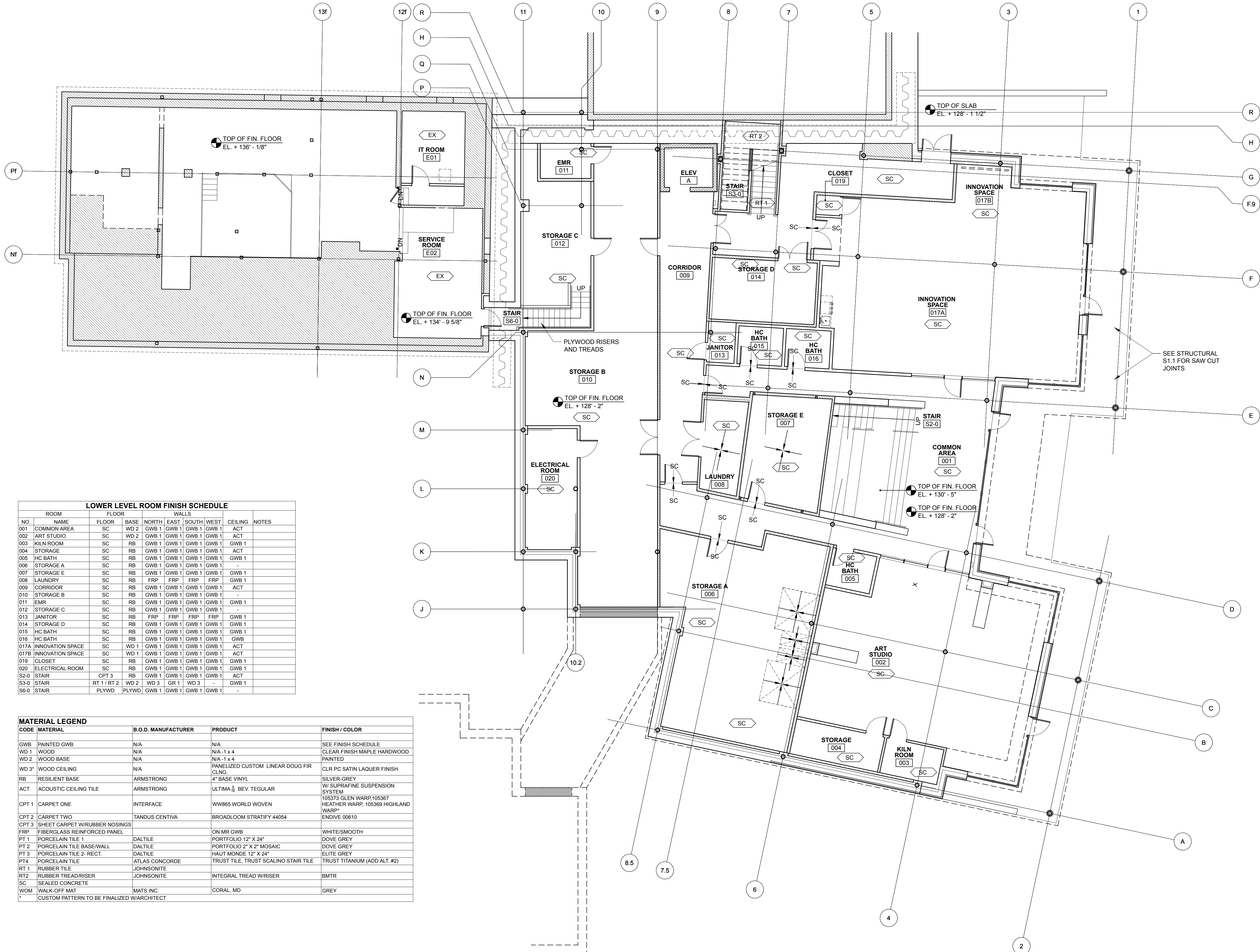
1 LOWER LEVEL FINISH PLAN SCALE: 1/8" = 1'-0"
