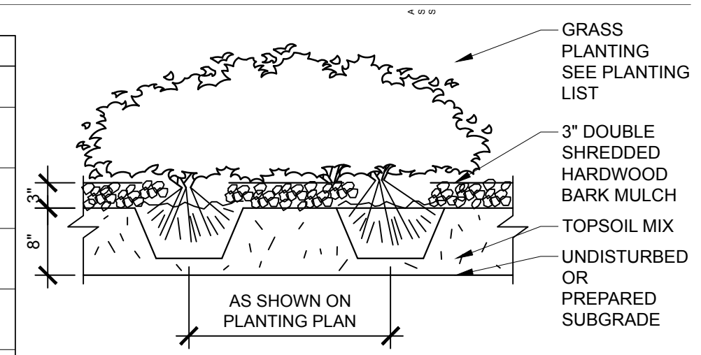
3 GROUND COVER DETAIL SCALE: 3/4" = 1'-0"
