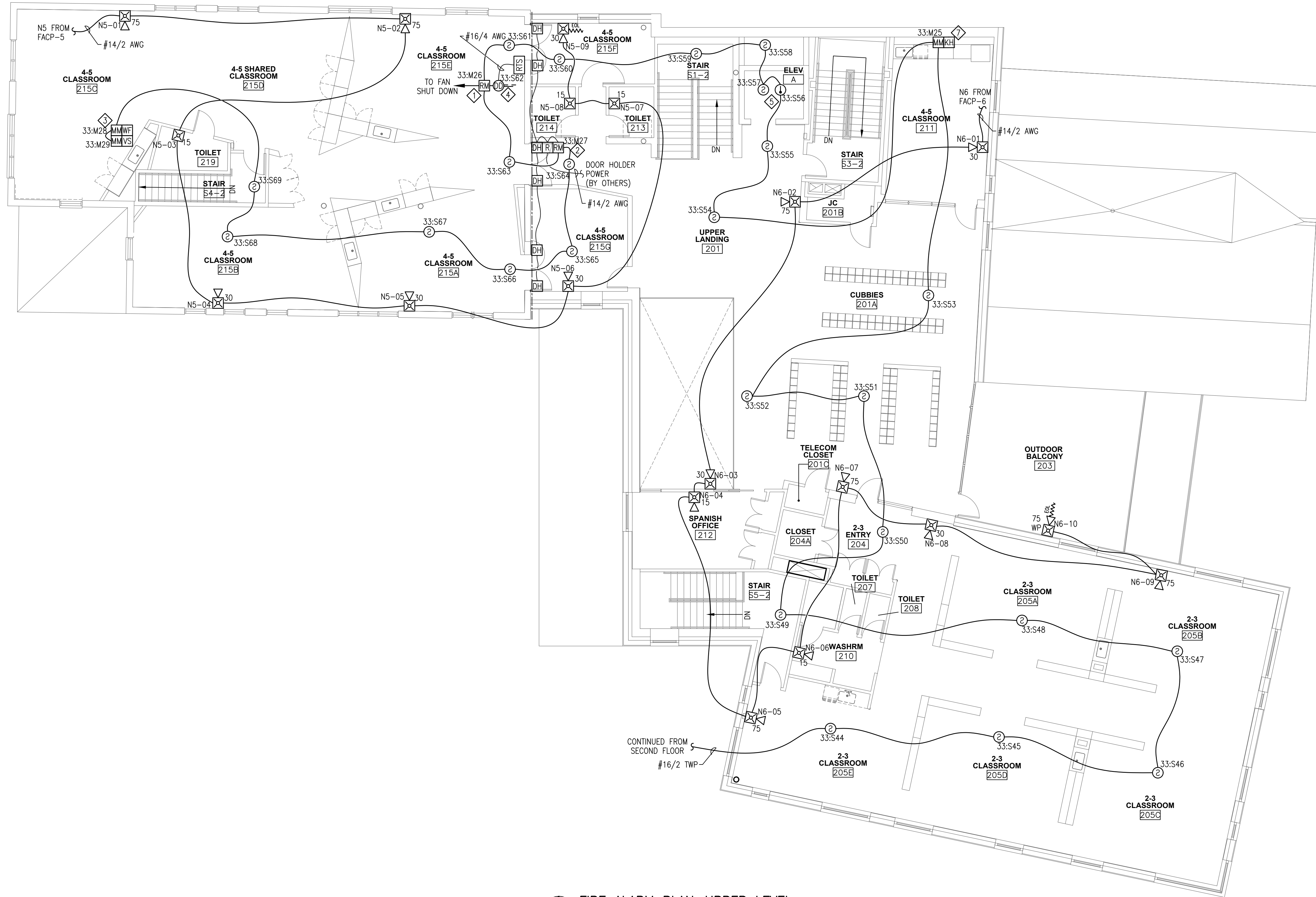
FIRE ALARM PLAN—UPPER LEVEL SCALE: 1/8"=1'-0"
