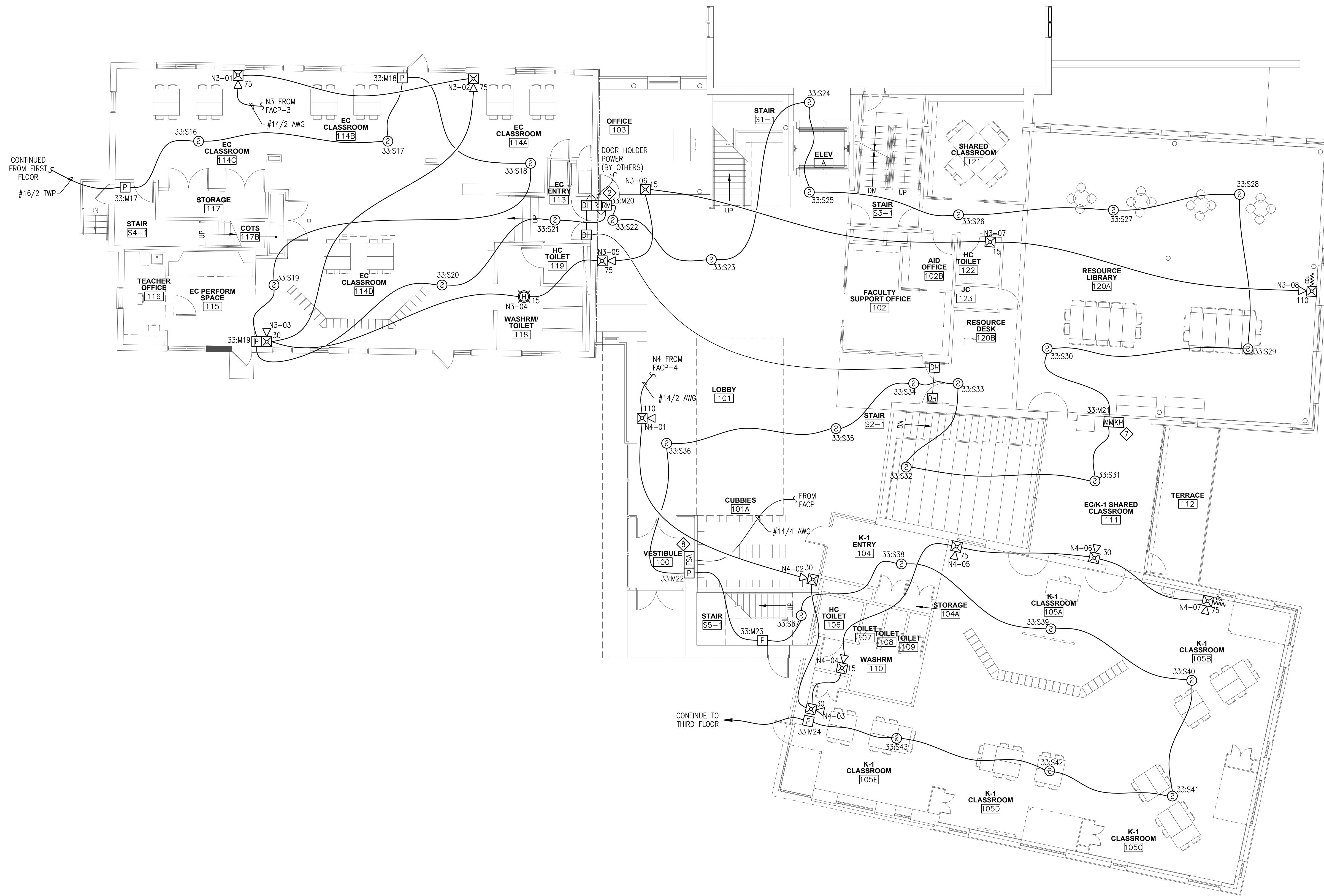
FIRE ALARM PLAN—MAIN LEVEL SCALE: 1/8"=1'-0"
