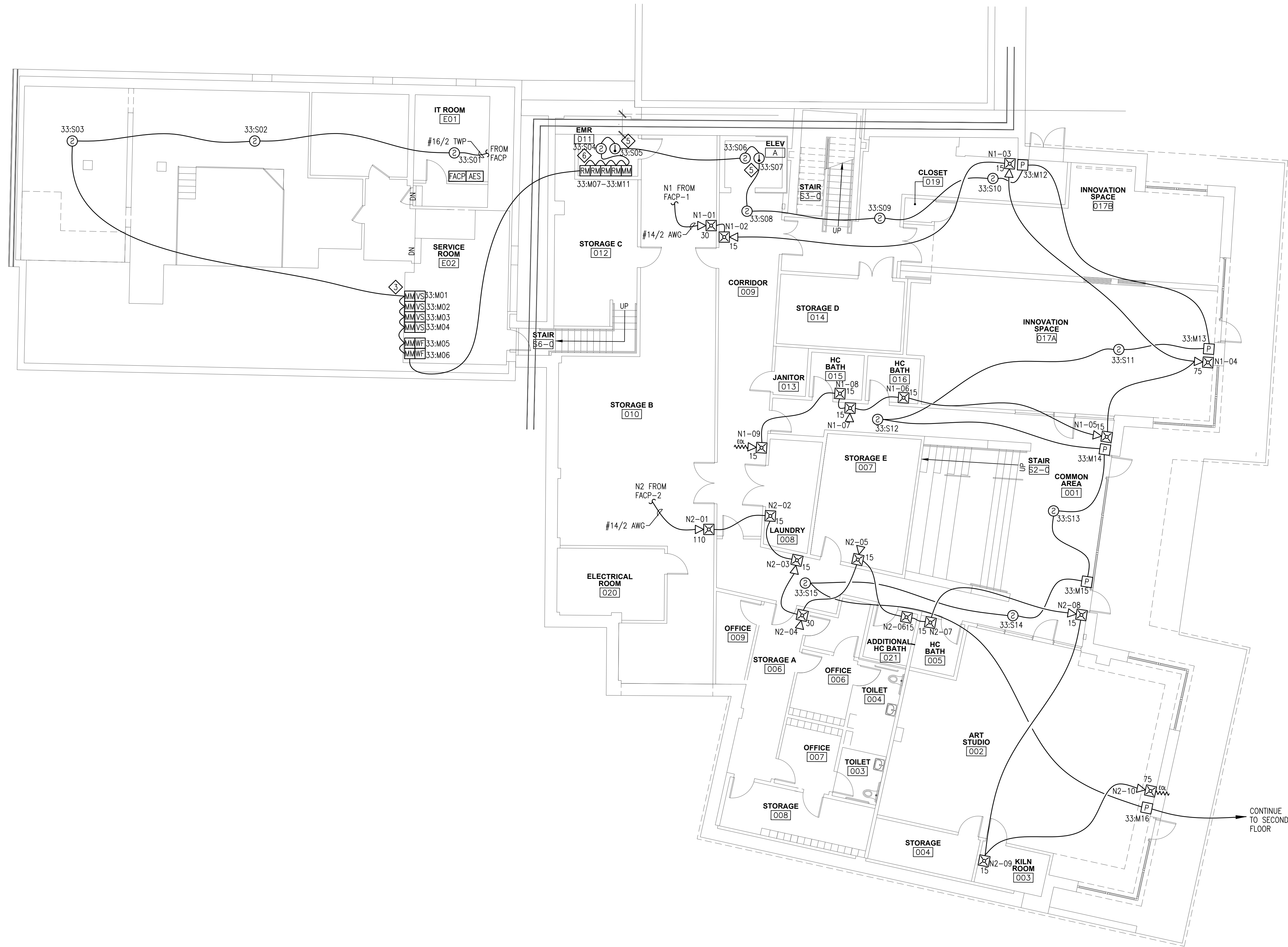
FIRE ALARM PLAN—LOWER LEVEL SCALE: 1/8"=1'-0"
