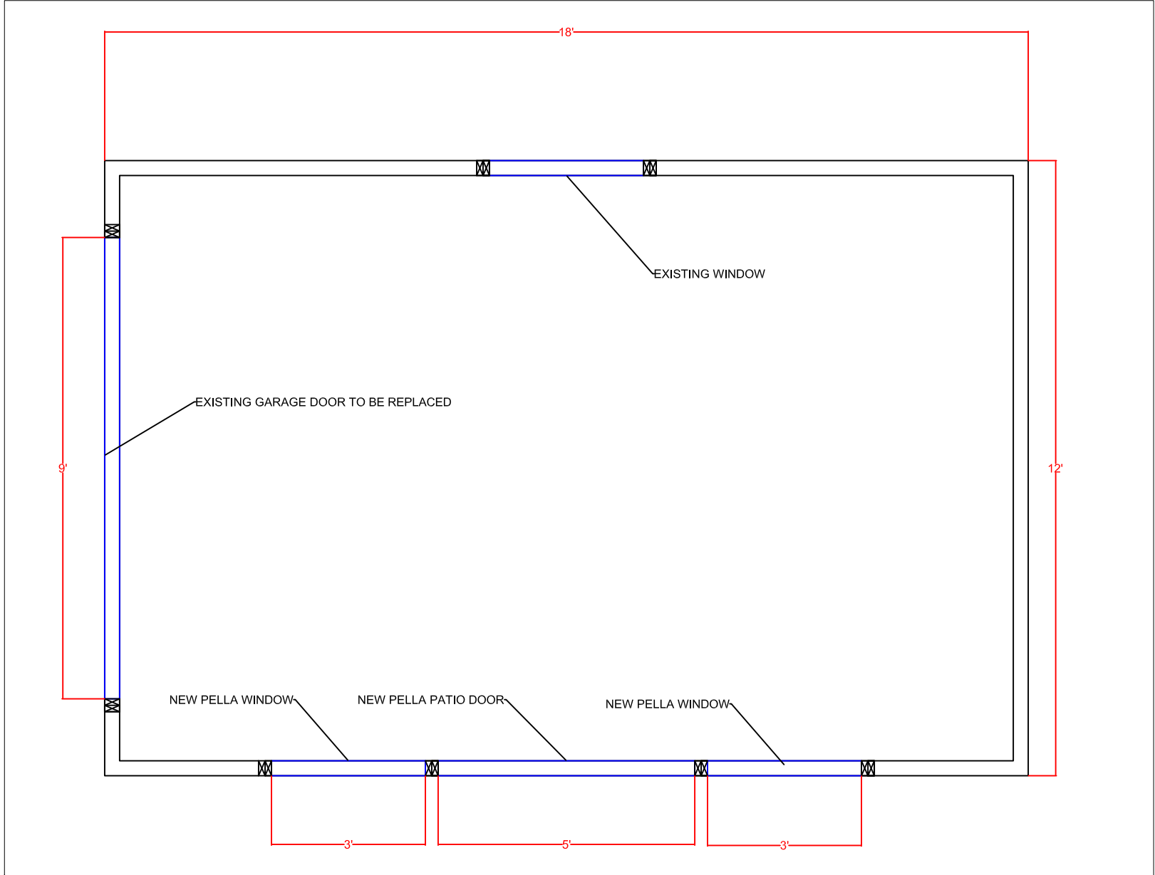
SECTION \frac{3}{8}'' = 1'-0''
