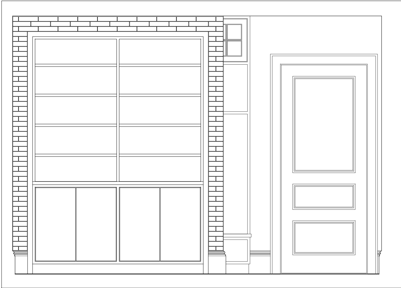
5 PANTRY ELEVATION SCALE: 1/2" = 1'-0"
